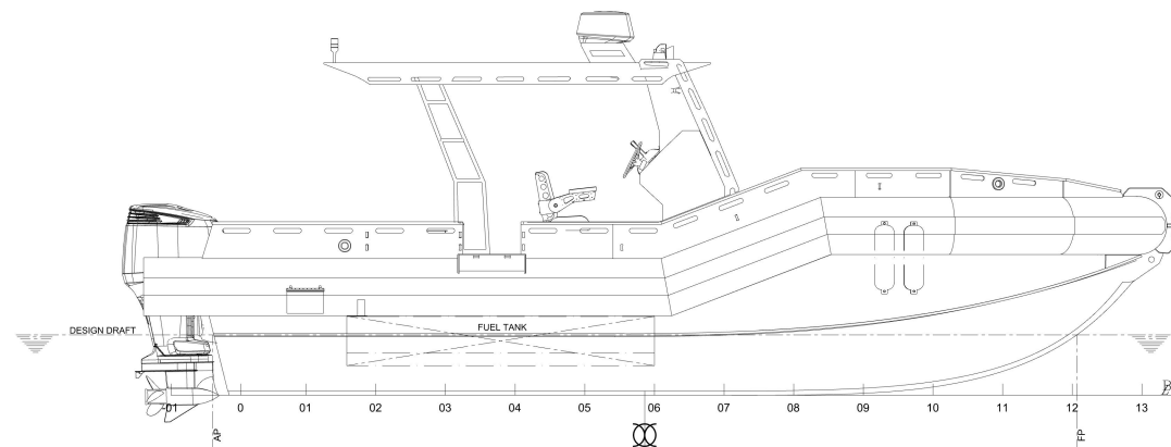
PROFILE VIEW
