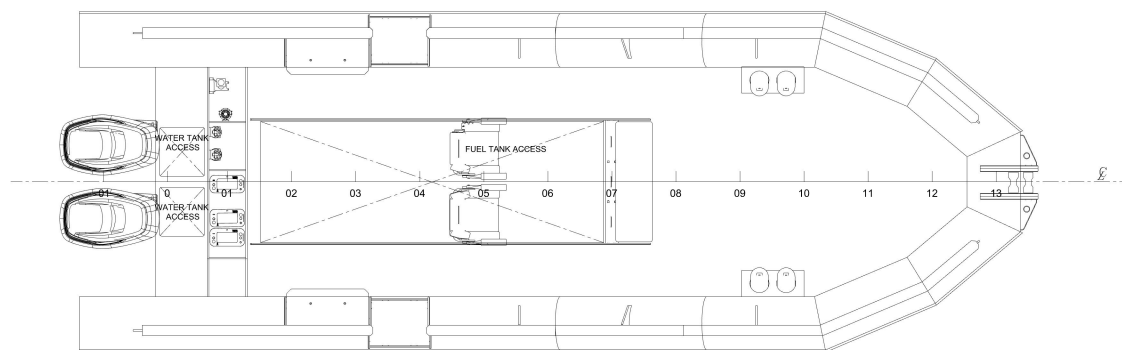
DECK VIEW
