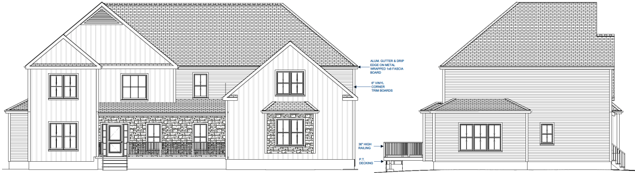
Front Elevation scale: 1/4" = 1'
