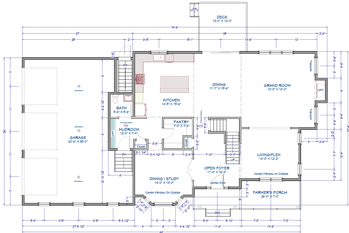
First Floor Plan scale: 1/3" = 1'
