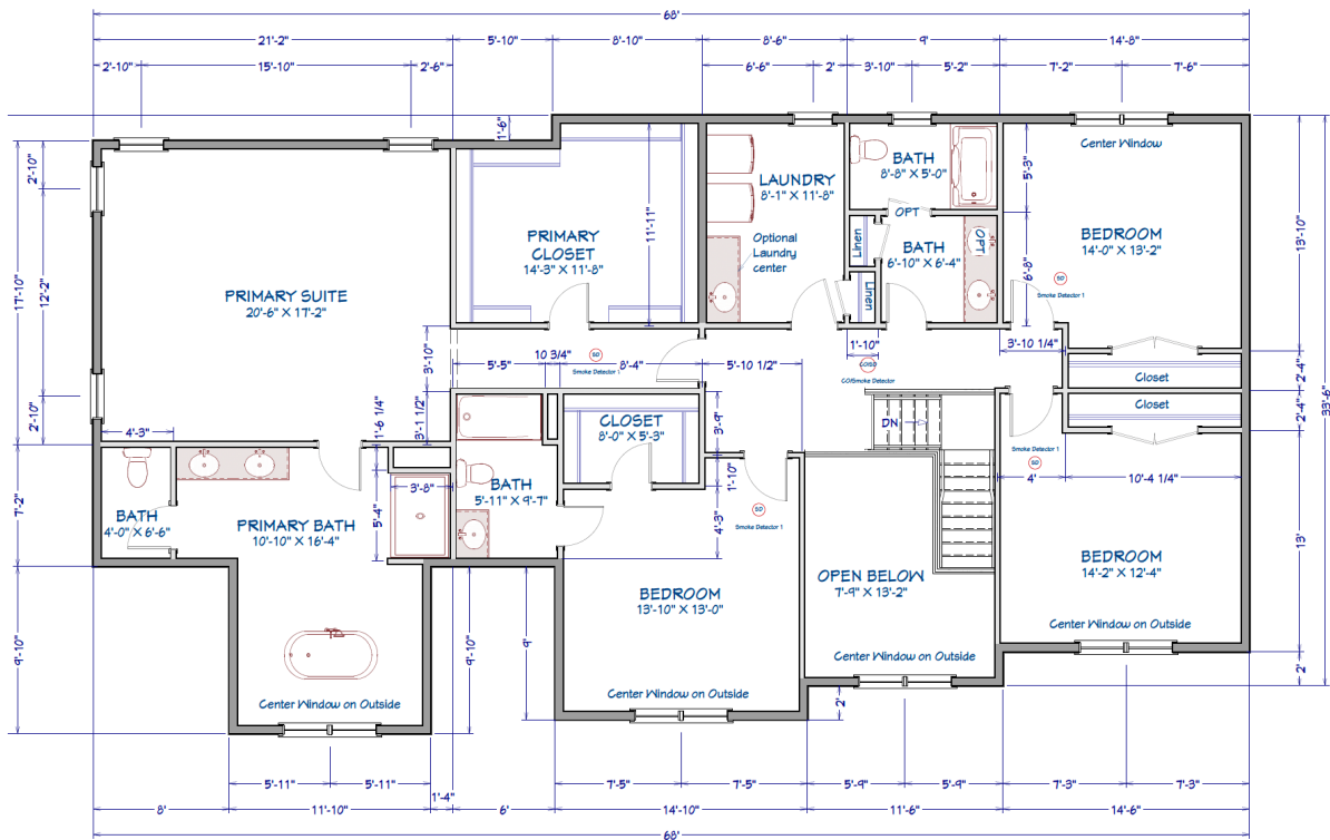
Second Floor Plan scale: 1/3" = 1'
