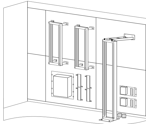
ReadySPEC® 9' Wall Kit (Racks and equipment not included)
