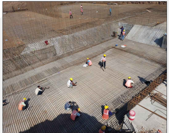
Homogeneous Tank (Under Progress)
