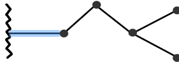
isopentil
