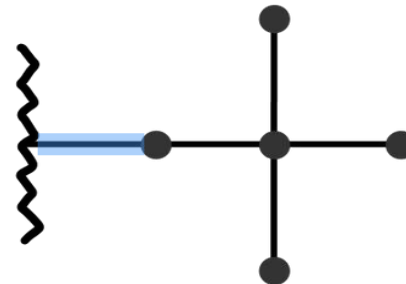
neopentil
