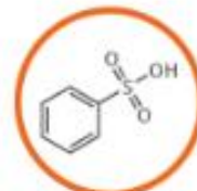
BENZENESULFONIC ACID Benzenesulfonic Acid C_6H_5SO_3H
