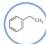
ETHYLBENZENE Ethylbenzene C_8H_{10}
