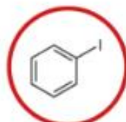
IODOBENZENE Iodobenzene C_6H_5I
