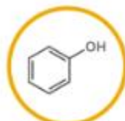
PHENOL Hydroxybenzene C_6H_5OH
