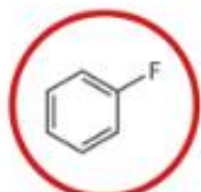
FLUOROBENZENE Fluorobenzene C_6H_5F
