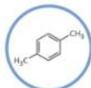
PARA-XYLENE 1,4-dimethylbenzene C_8H_{10}
