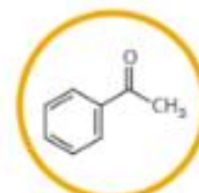
ACETOPHENONE 1-phenylethanone C_6H_5COCH_3
