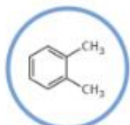
ORTHO-XYLENE 1,2-dimethylbenzene C_8H_{10}
