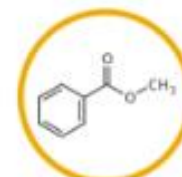
METHYL BENZOATE Methyl Benzoate C_6H_5CO_2CH_3
