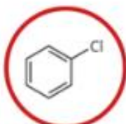
CHLOROBENZENE Chlorobenzene C_6H_5Cl
