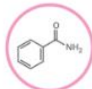
BENZAMIDE Benzamide C_6H_5CONH_2
