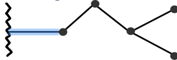
isopentil
