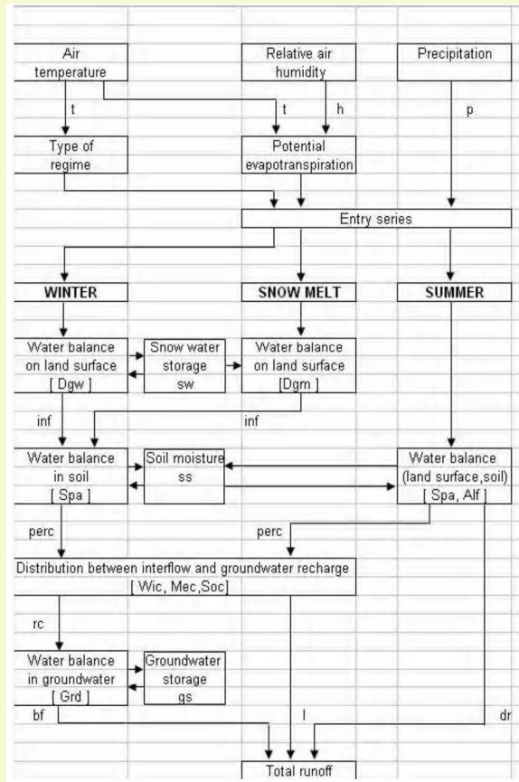
Figure 1. Internal structure of the BILAN water balance model
