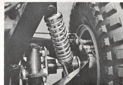
Heavy duty A-Frame suspension, service free U-Joints, self energizing brakes, dual shock on each wheel.
