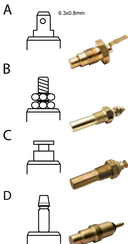
Temp Switch - Normally Open Contact - Single Terminal
