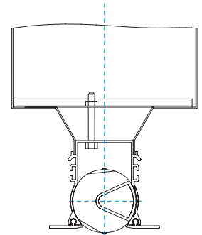
Fixing with a cross-member (Z)
