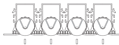
Every second row 1. Adjustment of deflectors for warm air supply
