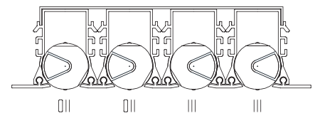
Every second row 2. Adjustment of deflectors for cold air supply
