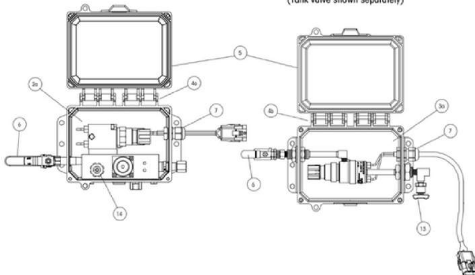
CP CONTROLLER ASSEMBLY (Tank valve shown separately)
