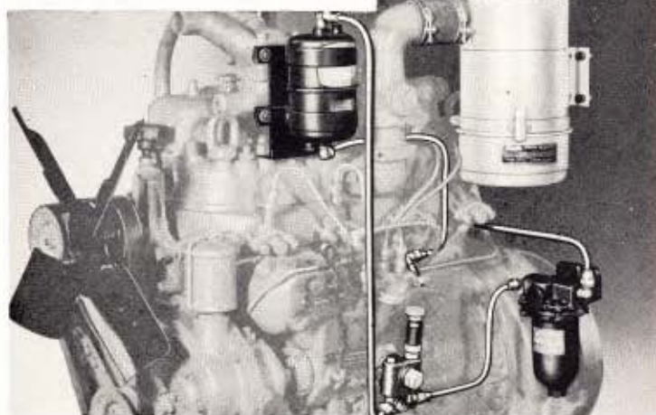
Fuel and oil filters on the Oliver "Cletrac" Diesel are not only highly efficient—they are placed where they are easily accessible.
