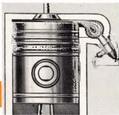
These are tolerances to fine in Oliver "Cletrac" Diesel engines that they can be measured only by a light gauge in terms of millionths of an inch.
