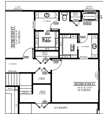
FLOOR PLAN @ OPTIONAL JACK AND JILL BATH
