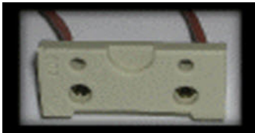
Ansi Code # H993 Socket for GY6.35 base types
