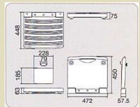
Product dimensions
