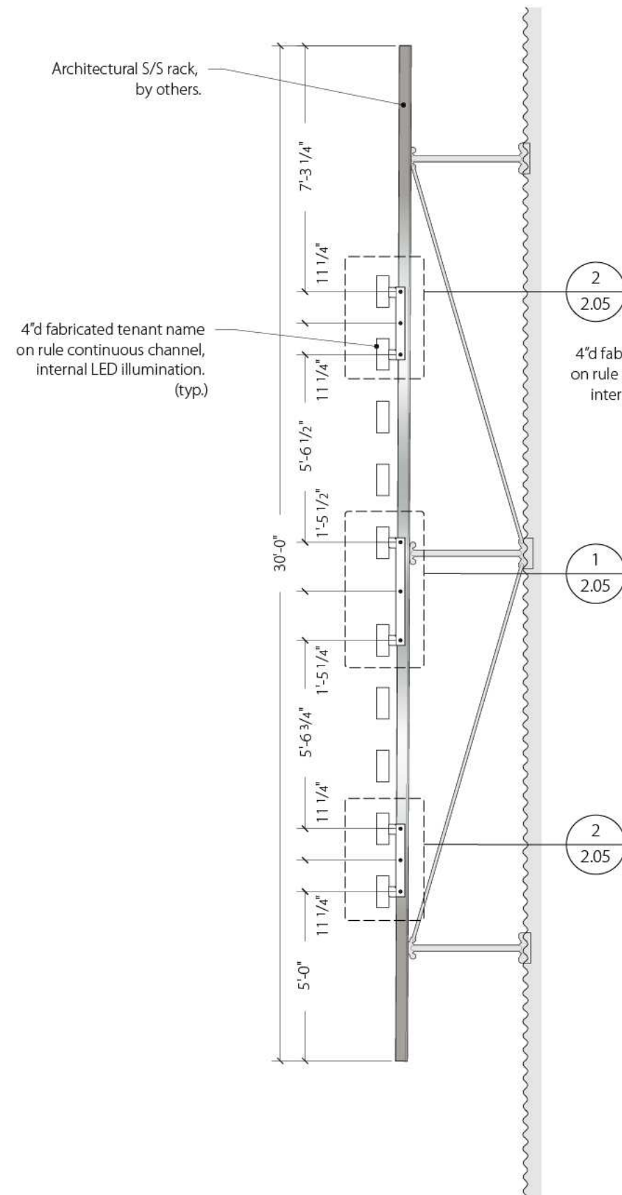
1 END VIEW, Project Logo Scale: 1/4" = 1'-0"
