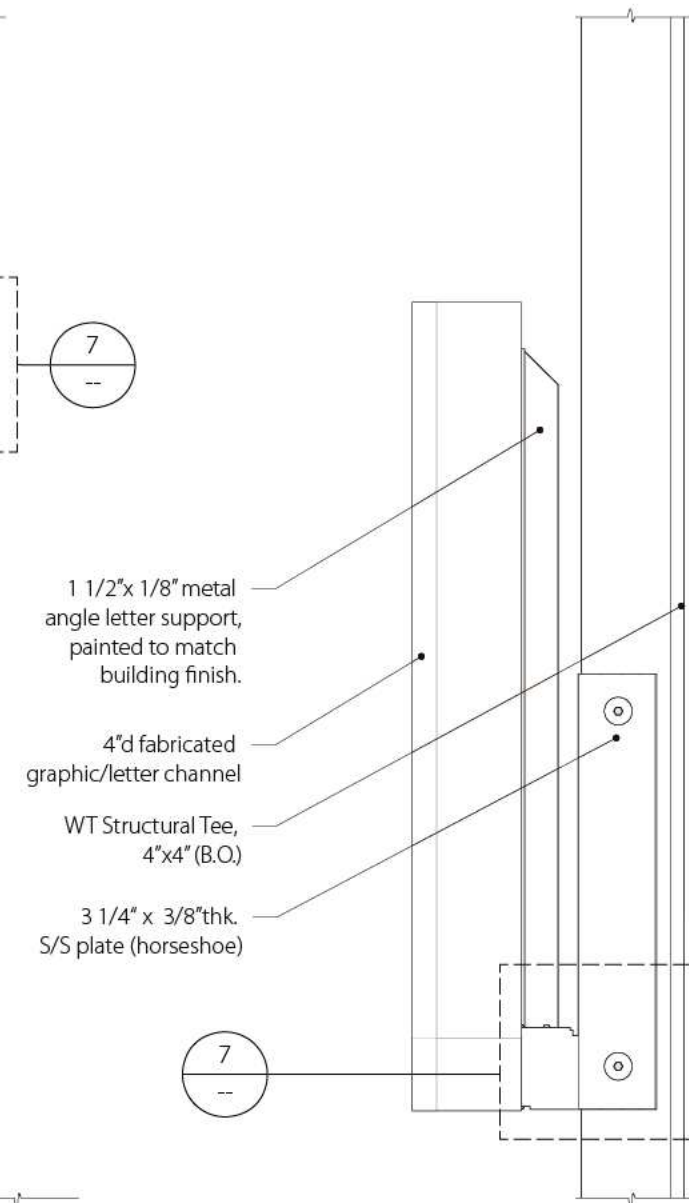
4 END VIEW, Tenant ID Scale: 1 1/2" = 1'-0"
