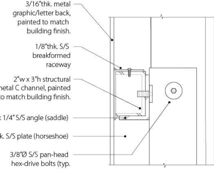
7 SECTION, Raceway Scale: 3" = 1'-0"
