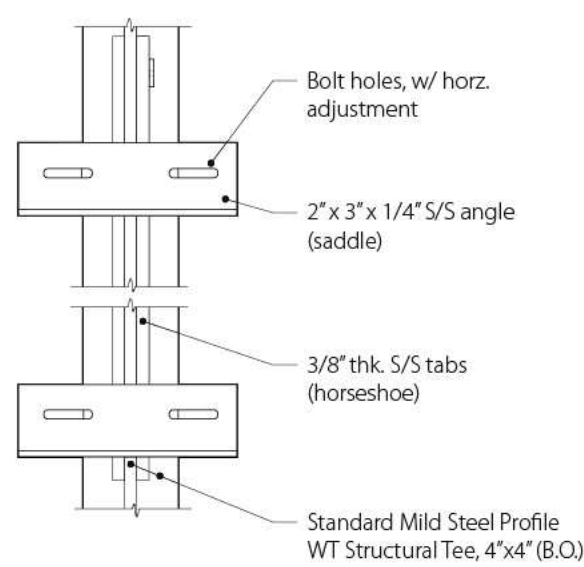
5 FRONT VIEW, Rack Bracket Scale: 1 1/2" = 1'-0"
