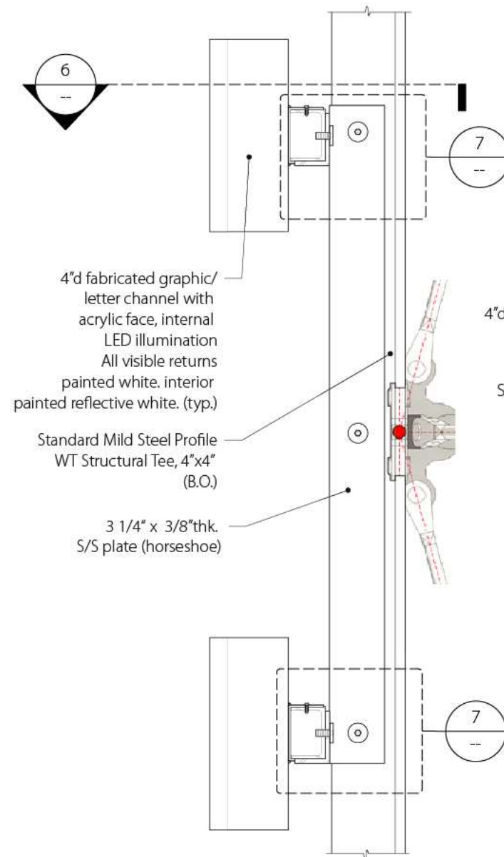
1 END VIEW, Logo Center Scale: 1 1/2" = 1'-0"
