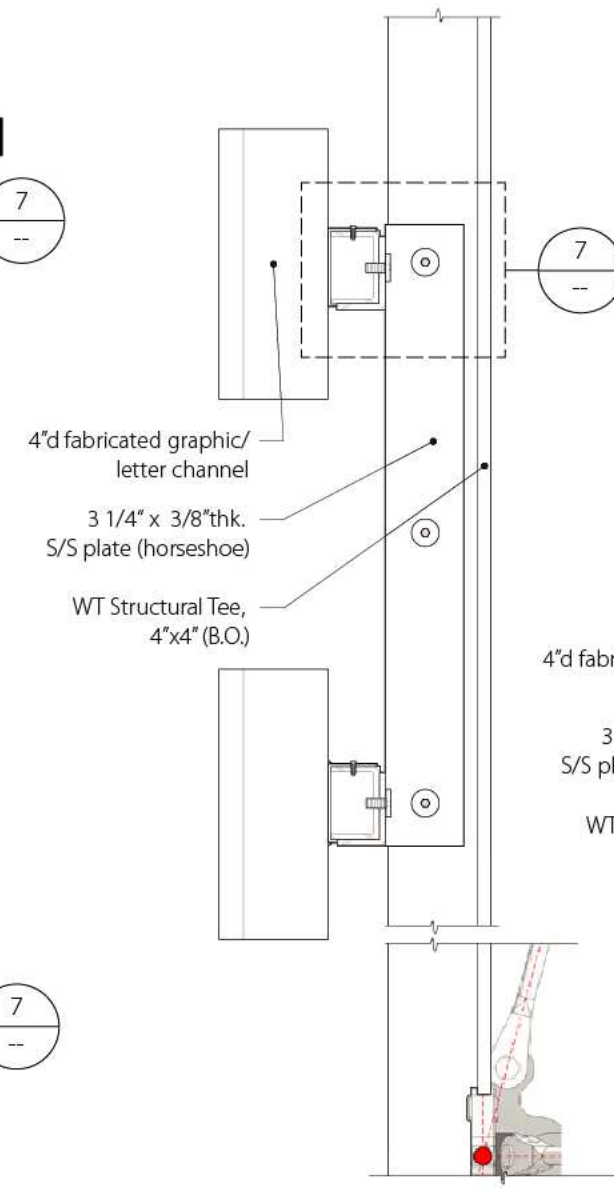
2 END VIEW, Logo Perimeter Scale: 1 1/2" = 1'-0"
