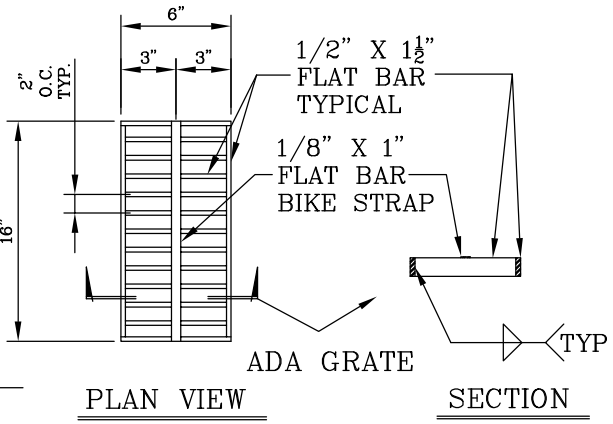
TYPICAL TRENCH GRATE ( 5 TOTAL FOR EACH TRENCH )
