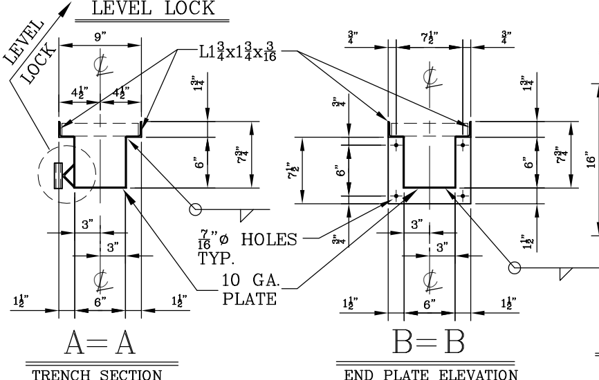
TYPICAL TRENCH GRATE ( 5 TOTAL FOR EACH TRENCH )
