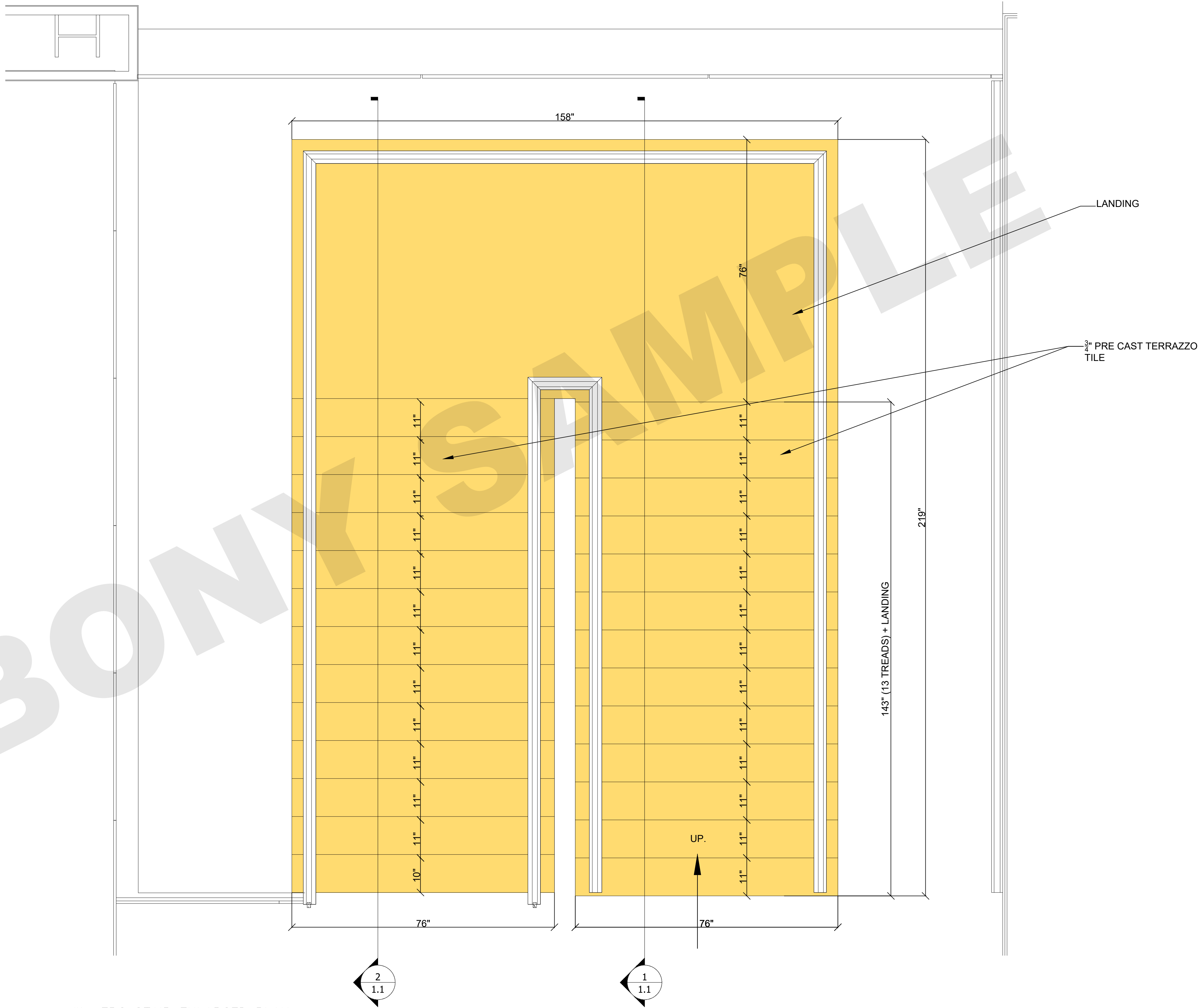
#1 EBC STAIR ENLARGED PLAN SCALE : \frac{3}{4} " = 1'-0"
