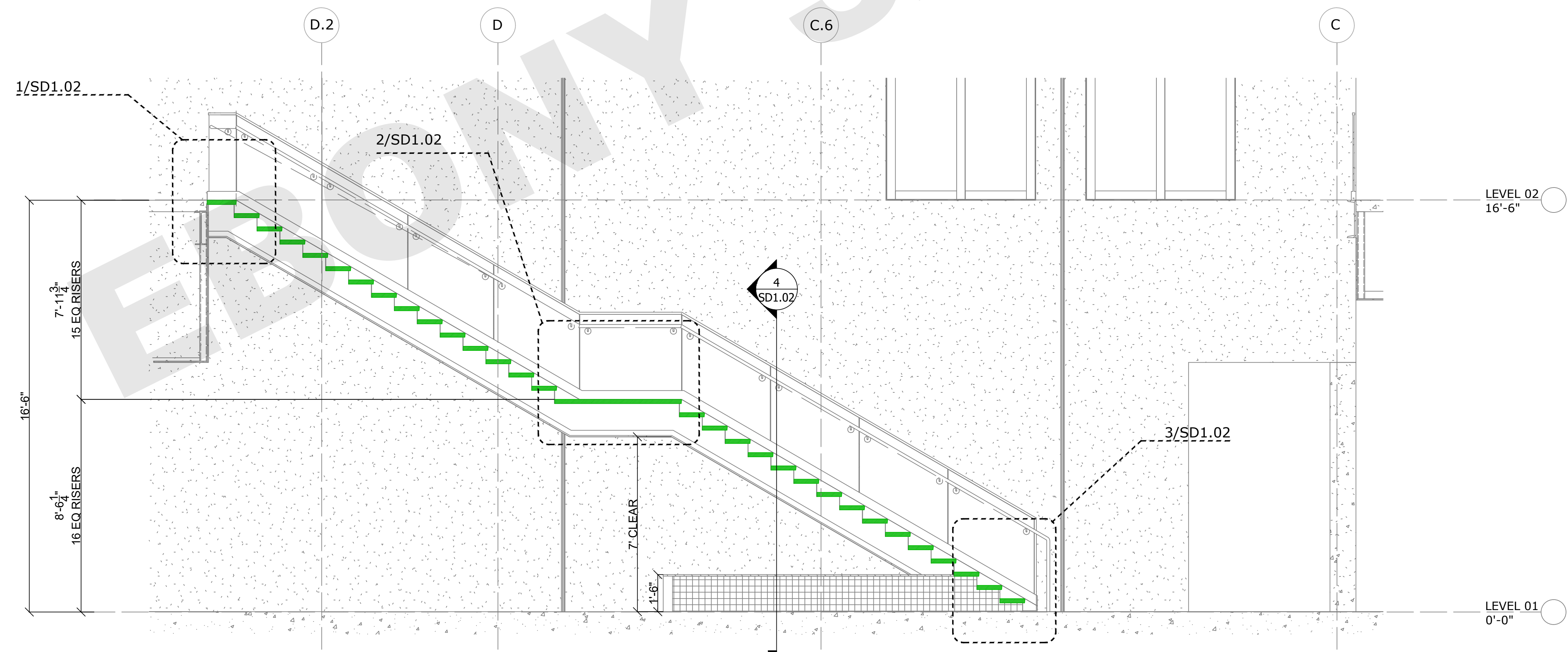
2 SECTION - LOBBY STAIR - SOUTH SCALE: 3/8"=1'-0" REF: 2/ A-442
