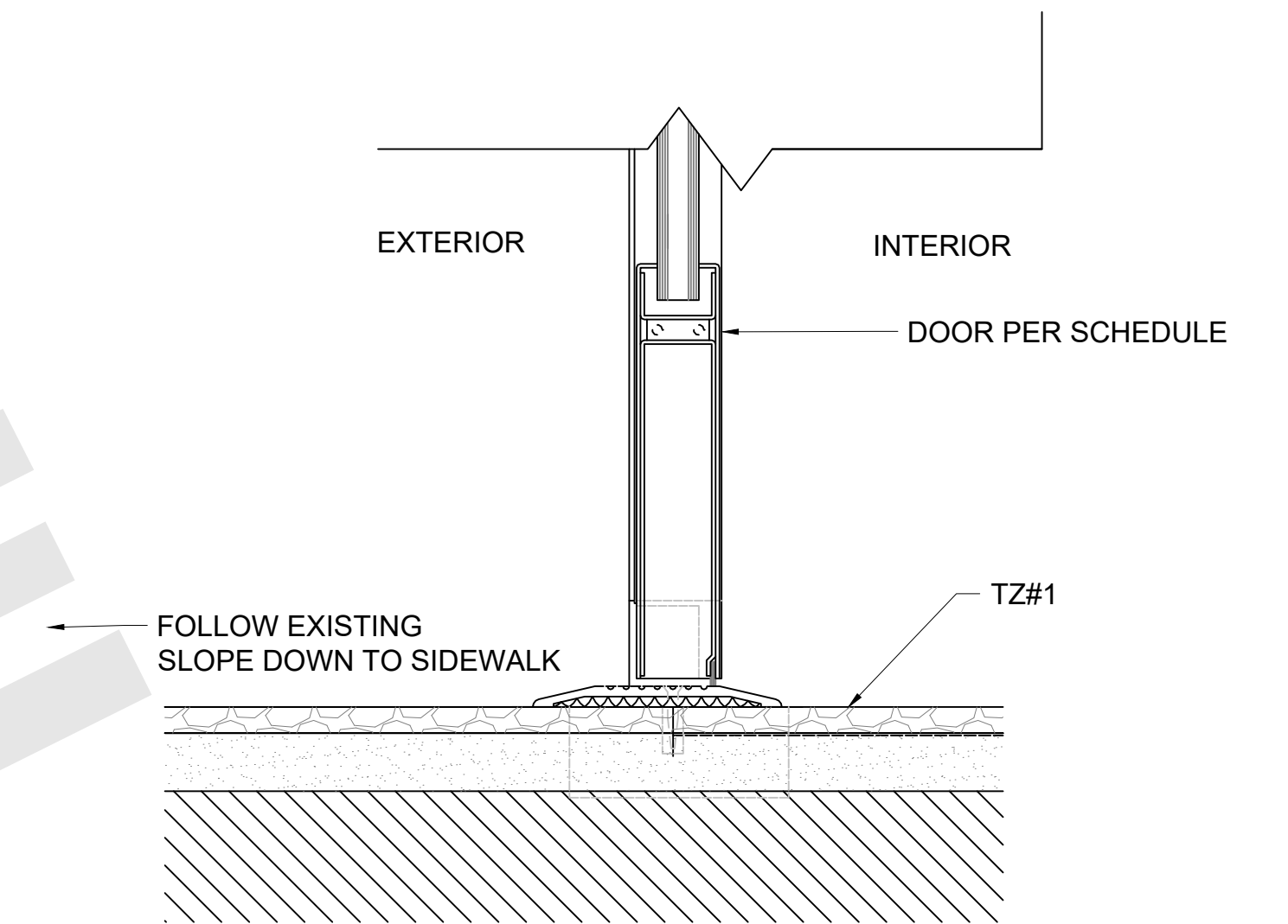
#4—THRESHOLD DETAIL DOOR 1
