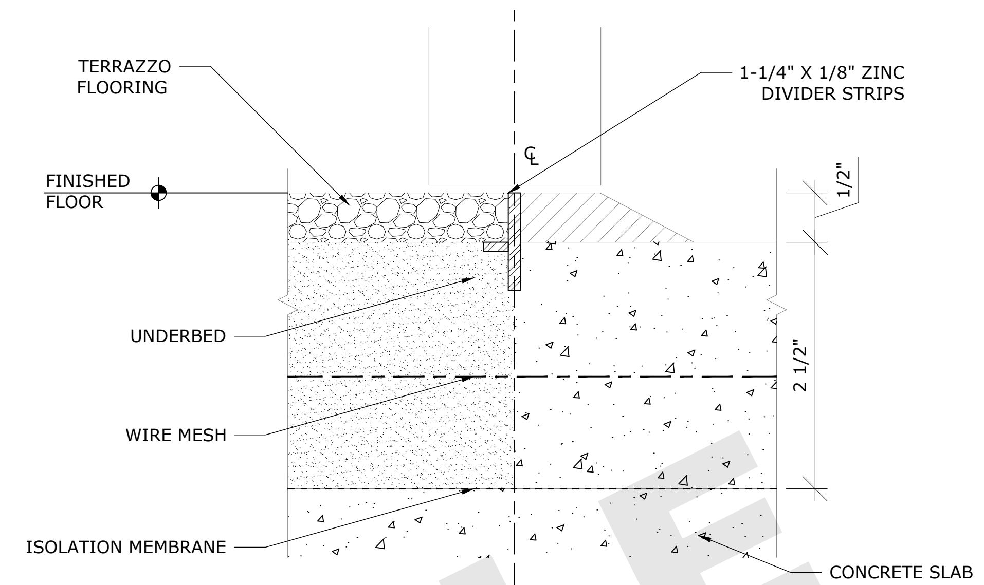
DIVIDER STRIP @DOOR TRANSITIONS
