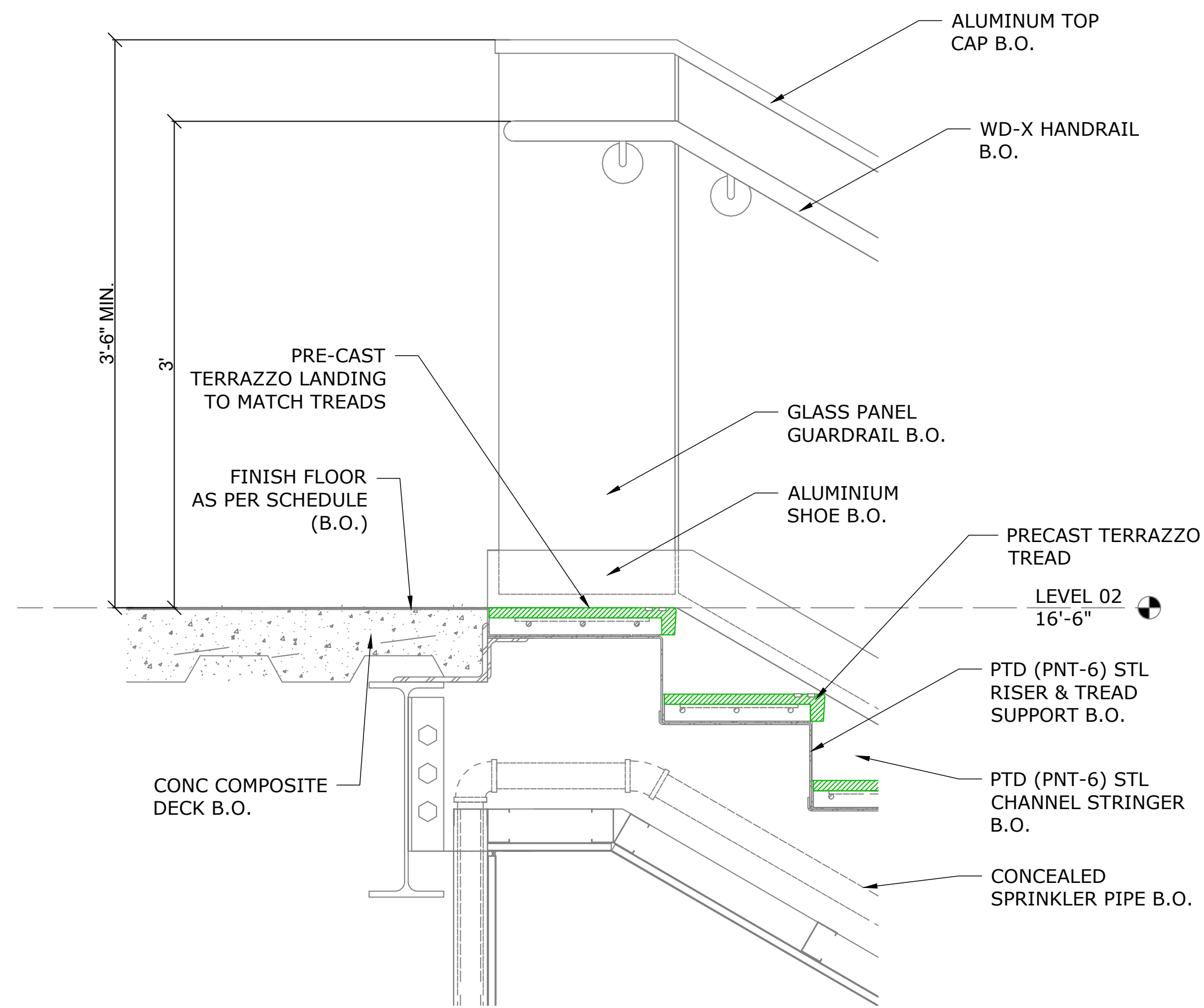
1 LOBBY STAIR TOP DETAIL SCALE: 1-1/2"=1'-0" REF: 6/ A-445
