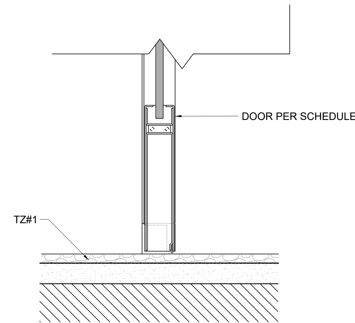
#1—THRESHOLD DETAIL DOOR 2
