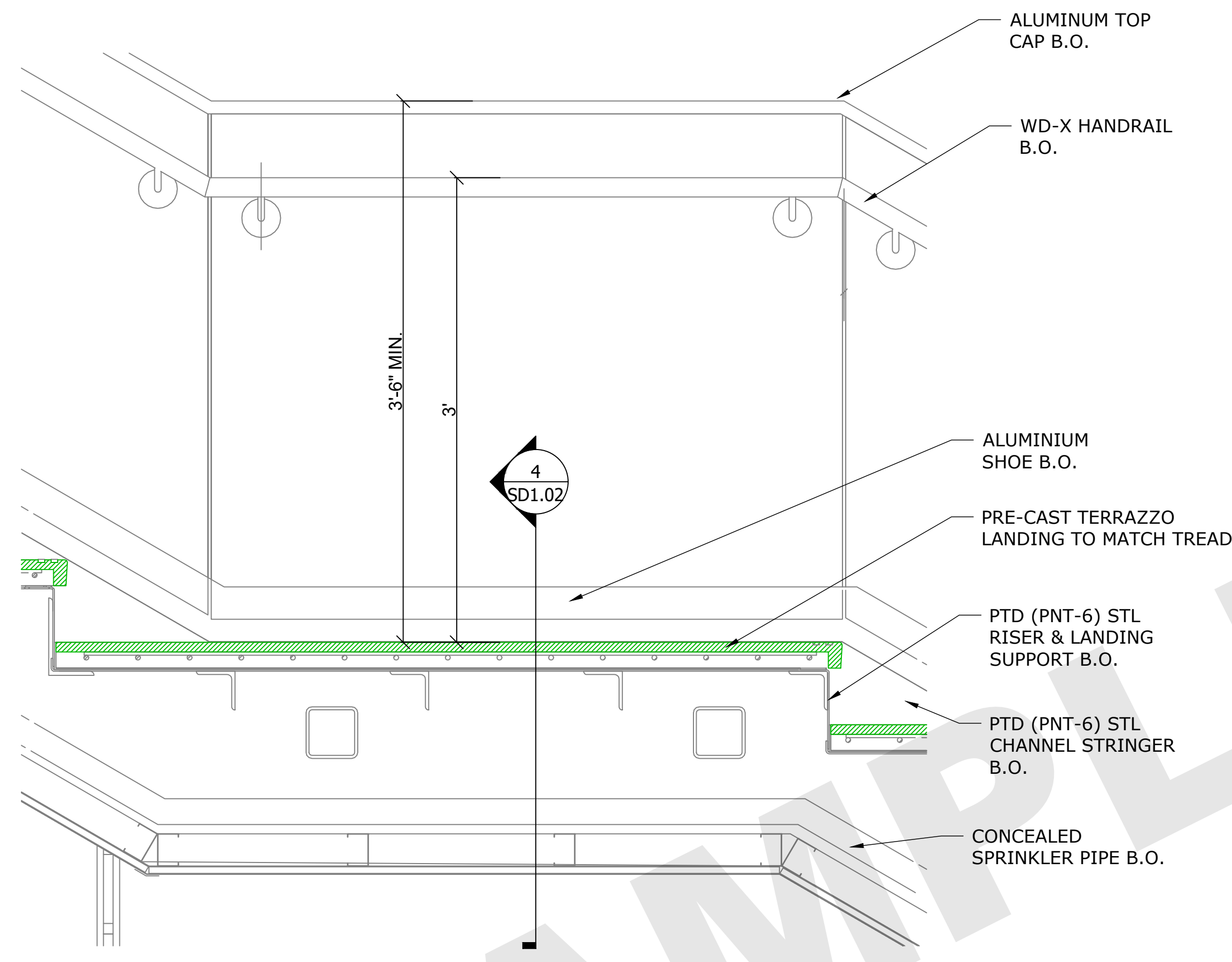
2 LOBBY STAIR LANDING DETAIL SCALE: 1-1/2"=1'-0" REF: 4/ A-445
