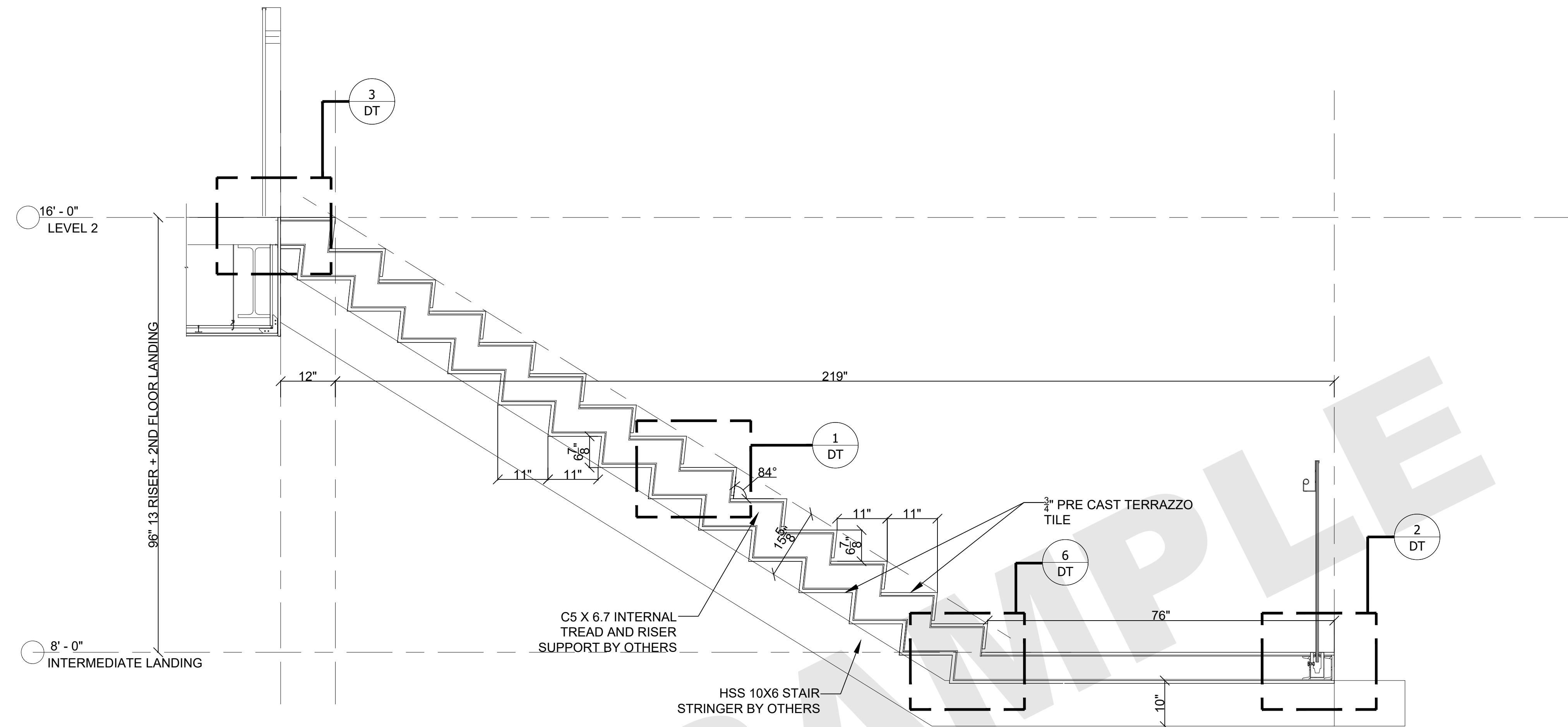
#2 EBC STAIR SECTION
