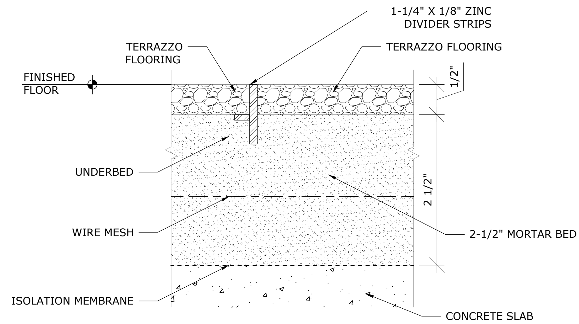
DIVIDER STRIP @FLOOR PATTERN
