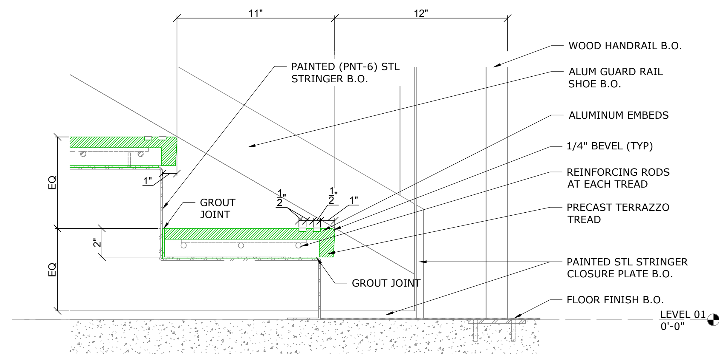
5 SECTION - LOBBY STAIR BOTTOM TREAD SCALE: 3"=1'-0" REF: 2/ A-444
