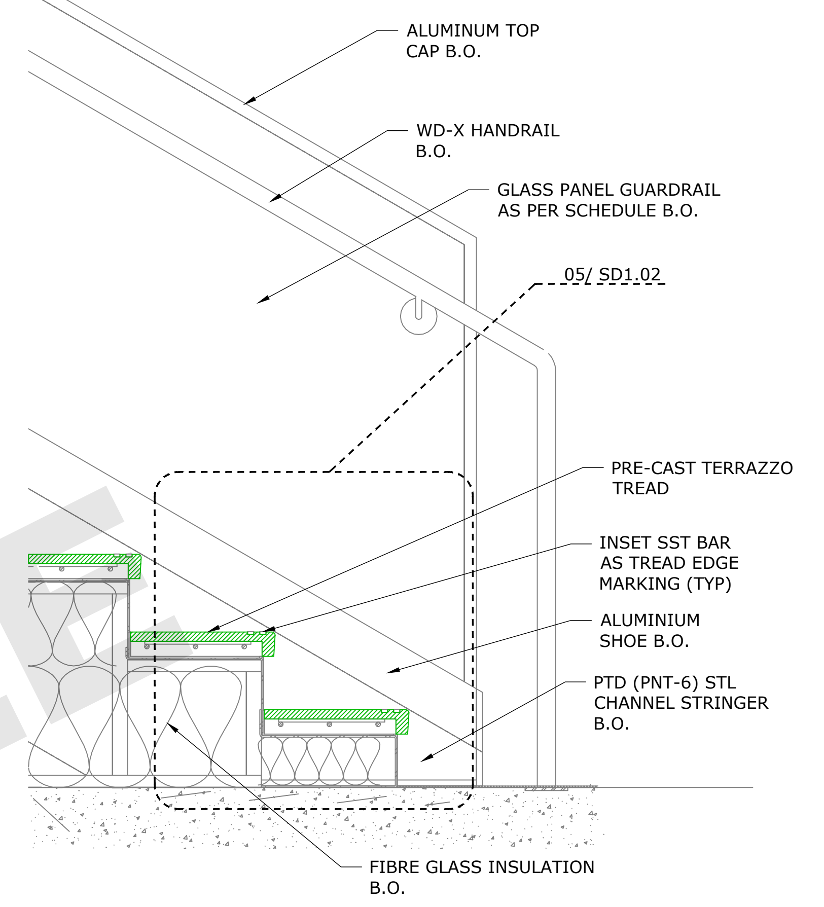
3 LOBBY STAIR BASE DETAIL SCALE: 1-1/2"=1'-0" REF: 1/ A-445
