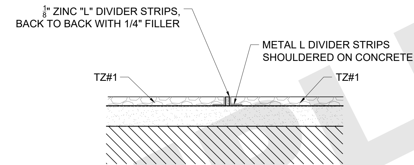
#3—DETAIL @ CONTROL JOINT
