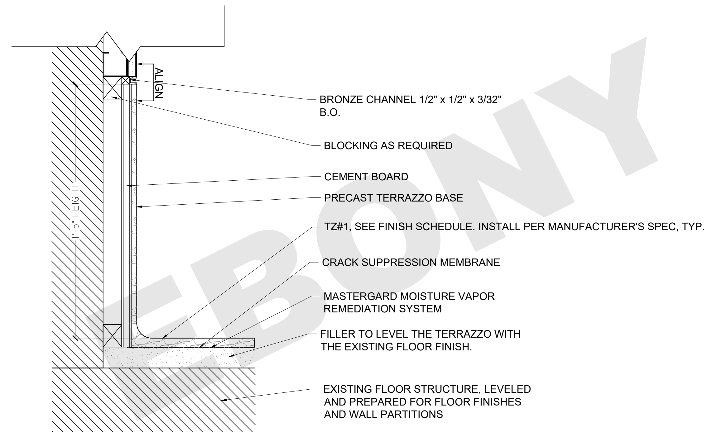
#1—THRESHOLD DETAIL— FLR#5 @ EXISTING FLOOR FINISH
