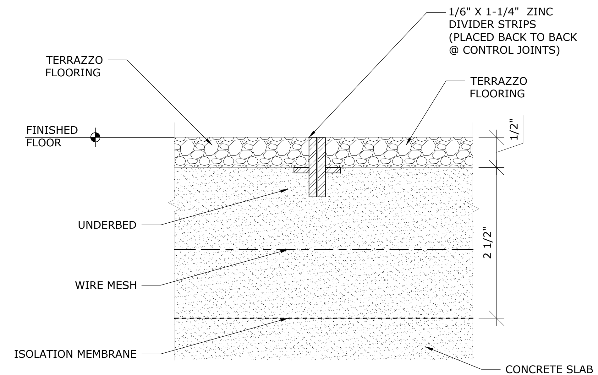
DIVIDER STRIP @CONTROL JOINTS
