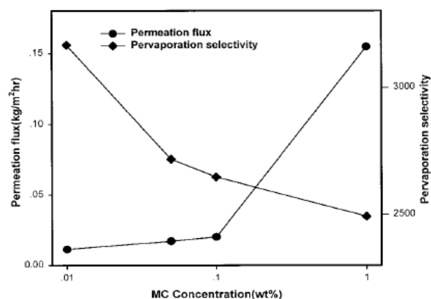
Fig. 5. Effect of the concentration of the organic compound (MC) on permeation flux and pervaporation selectivity of PSI membranes at 30°C [17].
