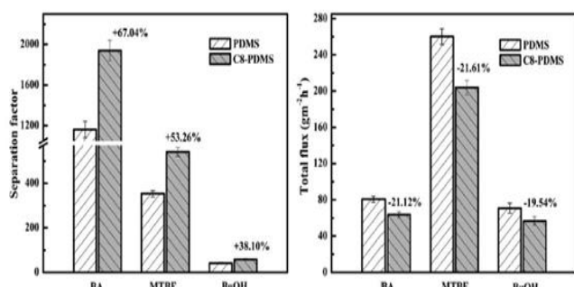
Fig. 7. Effect of alkyl grafting of C8-PDMS on separation factor and total flux for the treatment of different VOCs from water [20].
