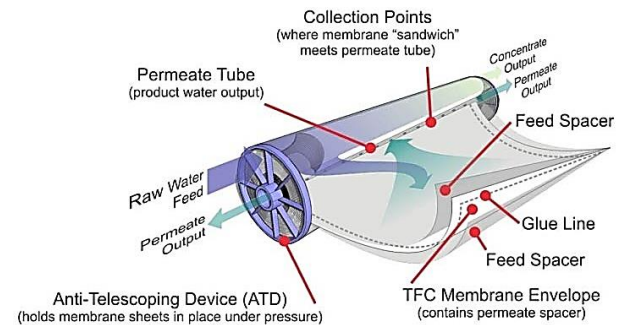
Fig. 1: Spiral-wound RO membrane configuration; Adapted from (AXEON, 2015)
