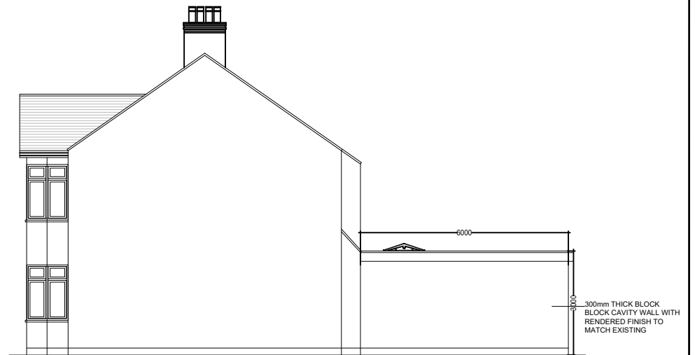
PROPOSED SIDE ELEVATION B
