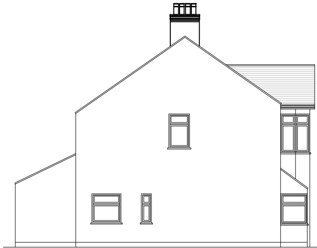
EXISTING SIDE ELEVATION A
