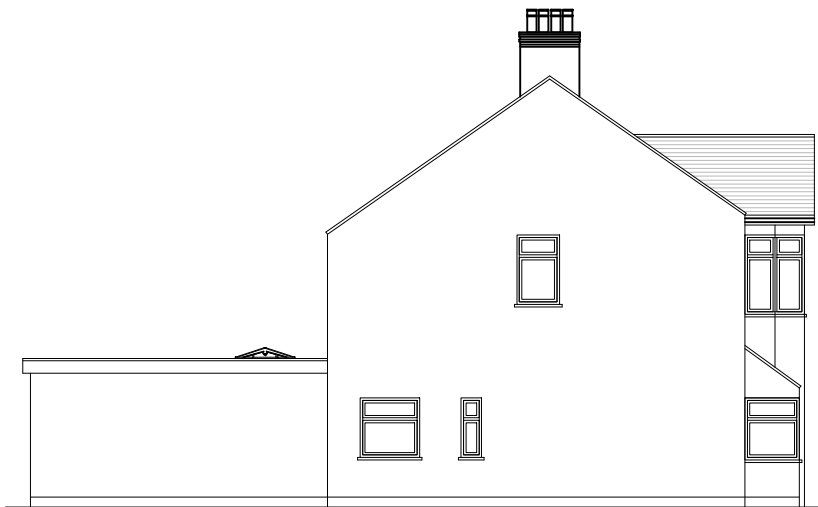
PROPOSED SIDE ELEVATION A
