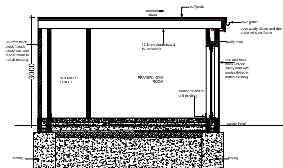
PROPOSED SECTION B
