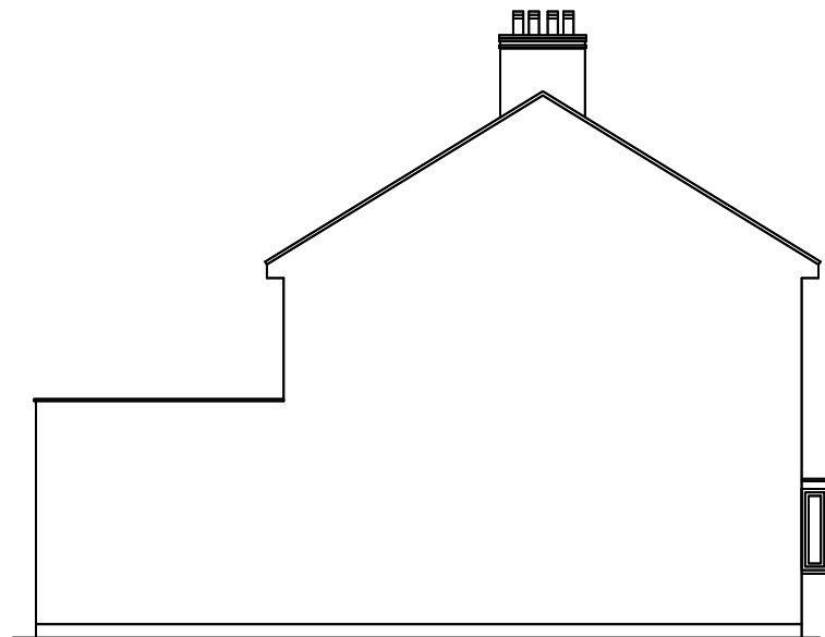
EXISTING SIDE ELEVATION A
