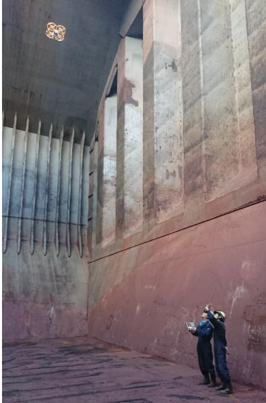
(Right) Underwater Drone (Left) Trial inspection of Aerial Drone in a cargo hold
