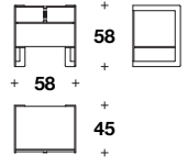
Bedside table w/ 2 drawers: VCM (11GL) - VCM (11GE) L: 58 (23") D: 45 (17 3/4") H: 58 (23")
