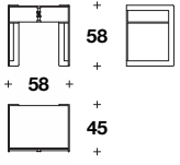
Bedside table w/ 1 drawer: VCM (10GL) - VCM (10GE) L: 58 (23") D: 45 (17 3/4") H: 58 (23")
