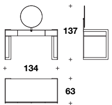
With optional mirror
