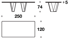
Rectangular table: VTB (26E) - VTB (26M) L: 250 (98 1/3") D: 120 (47 1/3") H: 74 (29") THK: 5 (1 15/16")
