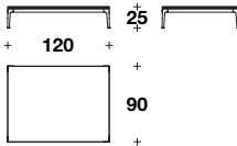
Low coffee table: VTC (12) L: 120 (47 1/3") D: 90 (35 1/3") H: 25 (9 3/4")
