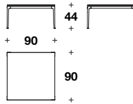
Coffee table: VTC (14) L: 90 (35 1/3") D: 90 (35 1/3") H: 44 (17 1/4")
