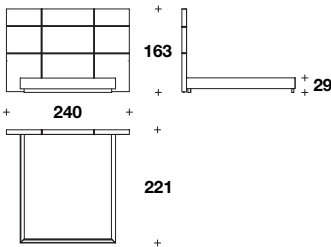
Bed for mattress 152x205 (60x80 2/3"): GRI (QUSA)
