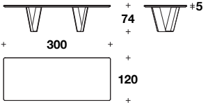
Rectangular table: VTB (27E) - VTB (27M) L: 300 (118") D: 120 (47 1/3") H: 74 (29") THK: 5 (1 15/16")
