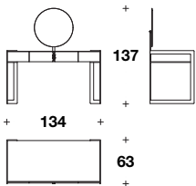
With optional mirror
