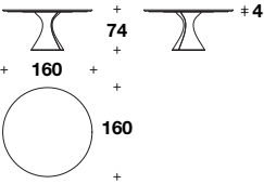
Round table: VTB (23) - VTB (23V) L-D: Ø 160 (Ø 63") H: 74 (29") THK: 4 (1 9/16")
