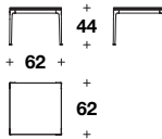
Coffee table: VTC (13) L: 62 (24 1/3") D: 62 (24 1/3") H: 44 (17 1/4")
