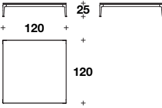
Low coffee table: VTC (11) L: 120 (47 1/3") D: 120 (47 1/3") H: 25 (9 3/4")
