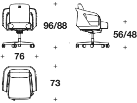
LOW CONFERENCE CHAIR: SBG (03B) L: 76 (30") D: 73 (28 2/3") H: 96-88 (37 2/3-34 2/3") HS: 56-48 (22-19")
