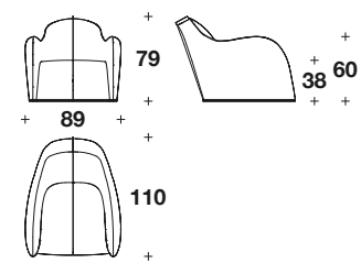
ARMCHAIR: BBP (01)
