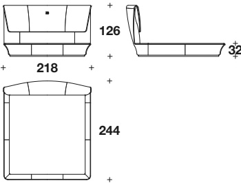
BED FOR MATTRESS 185x200 (73x78 2/3"): LEB (LE2)
