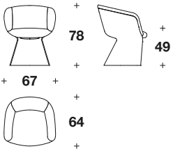
VITESSE SENSE CHAIR: SBG (06) L: 67 (26 1/3") D: 64 (25 1/3") H: 78 (30 2/3") HS: 49 (19 1/4")
