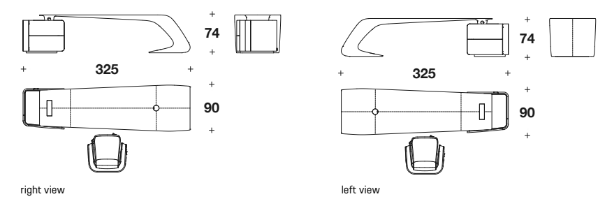
RIGHT OR LEFT DESK WITH SMALL DRAWERS: BTA (03PD) - BTA (03PS) L: 325 (128") D: 90 (35 1/3") H: 74 (29")
