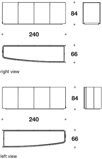
RIGHT OR LEFT LOW CABINET - 4 DOORS: MEB (01PD) - MEB (01PS)
