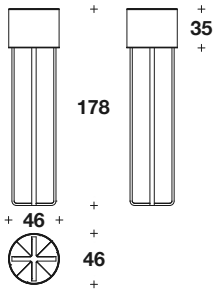
STANDING LAMP: LBU (01)
