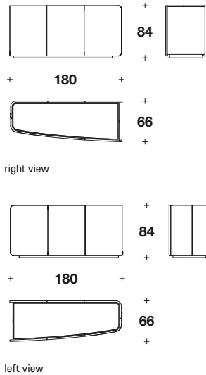
RIGHT OR LEFT LOW CABINET - 3 DOORS: MEB (02PD) - MEB (02PS)
