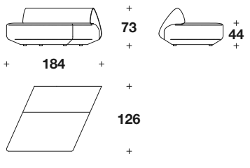
RIGHT OR LEFT CENTRAL ELEMENT: DBB (ECD) - DBB (ECS) Drawing: right element
