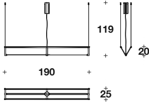
SUSPENSION: LBU (17)
