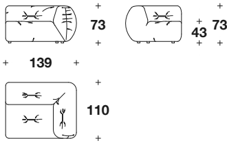
SEAT ELEMENT WITH RIGHT OR LEFT ARMREST: BOU (E1D) - BOU (E1S) Drawing: right element
