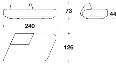
SEATER ELEMENT WITH RIGHT OR LEFT ARMREST: DBB (PEND) - DBB (PENS) Drawing: right element
