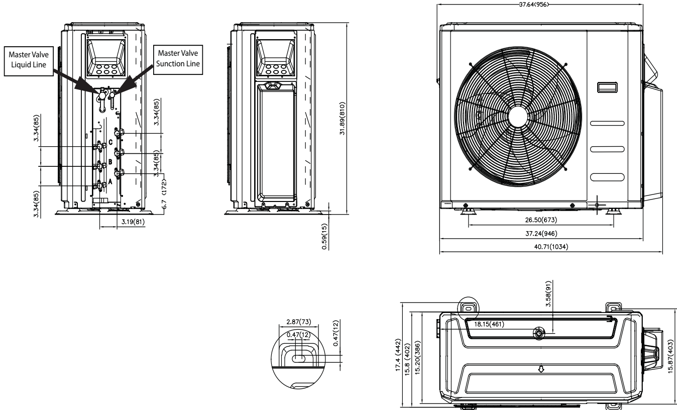
Fig. 5 – Outdoor Dimensions Size 27
