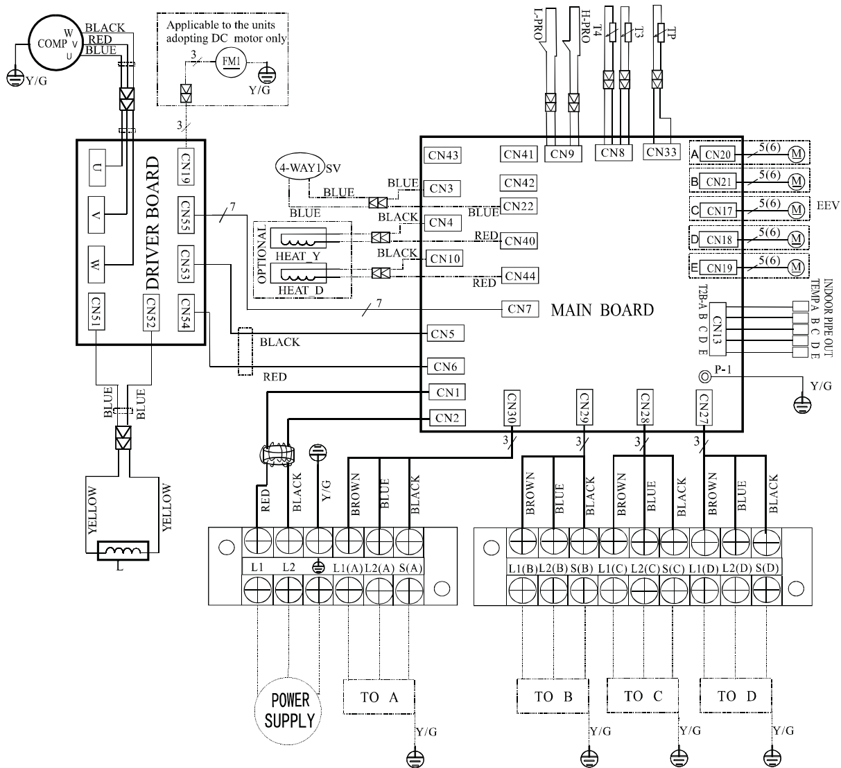
Fig. 13 – Wiring Diagrams 36K – 4 Zone Max
