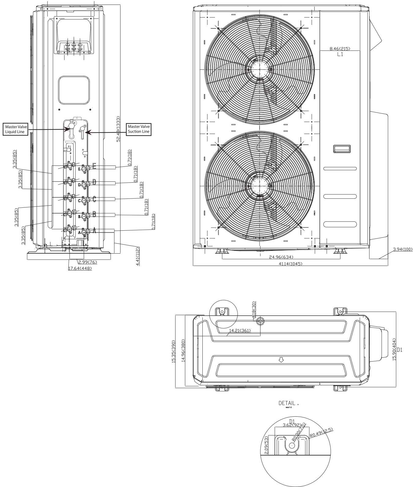
Fig. 7 — Outdoor Dimensions Size 48
