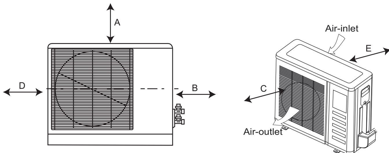
Fig. 8 – Clearances Outdoor
