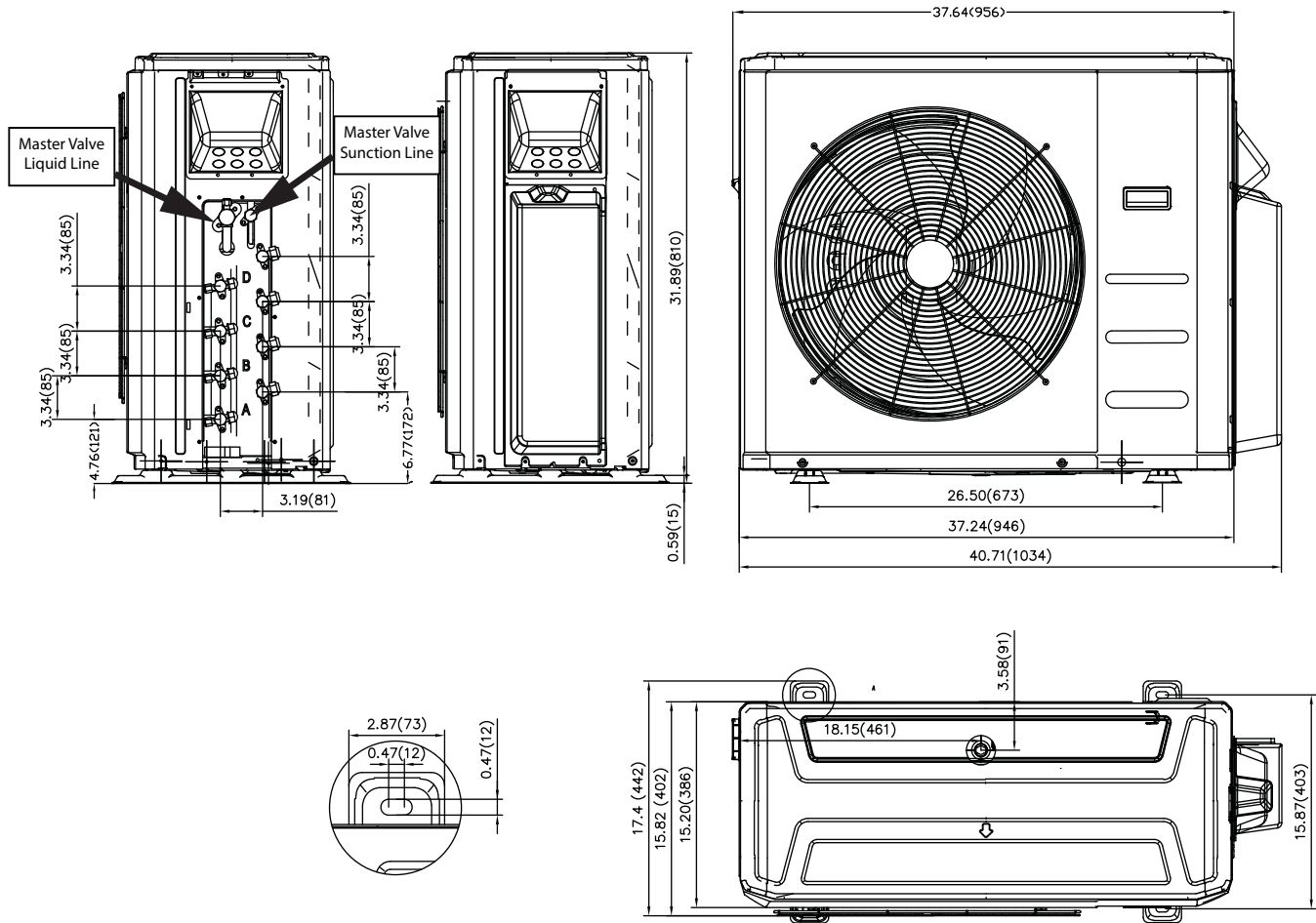
Fig. 6 – Outdoor Dimensions Size 36
