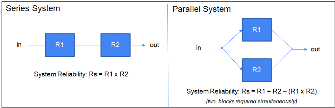
Diagram 2 – Illustrating basic RBDs and their reliability calculation equation
