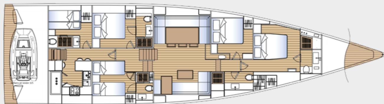
ALTERNATIVE INTERIOR PLANS.
