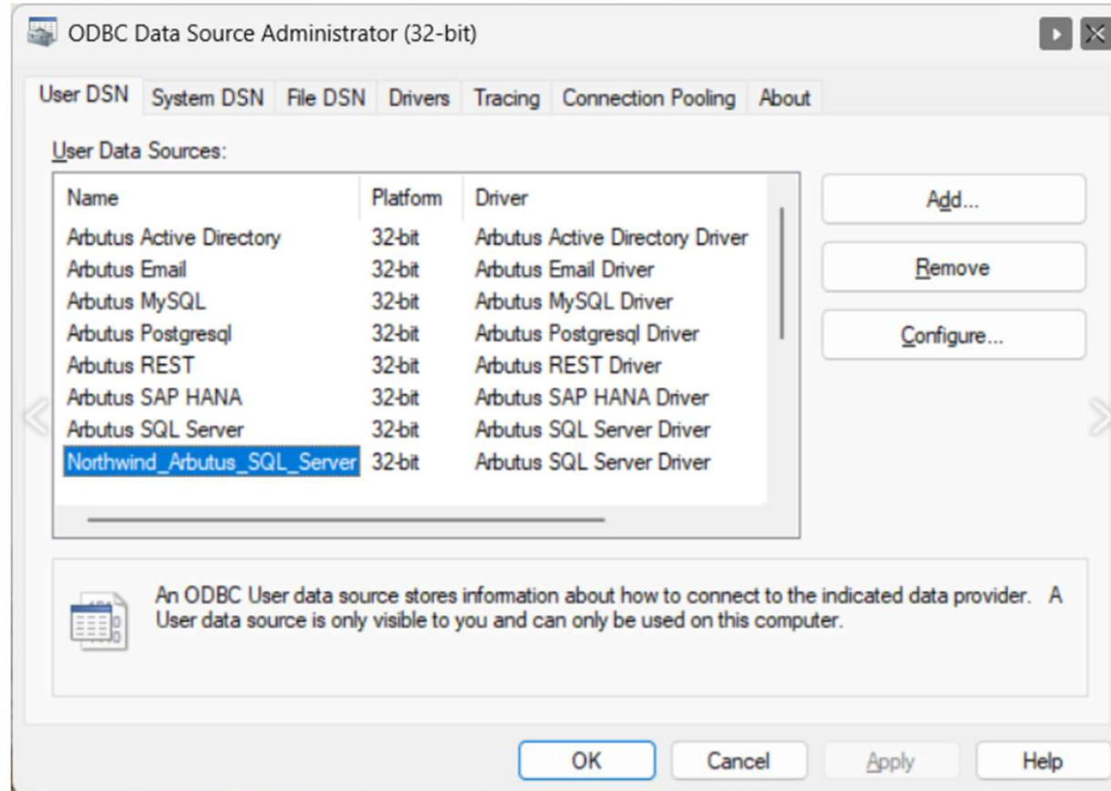
Arbutus Data Connectors as ODBC data sources Item 1 of 5
