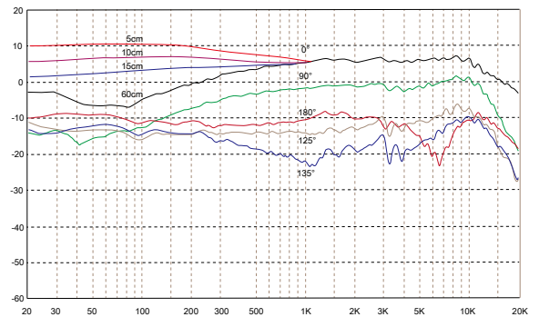
CSLC, super cardioid low roll off close pickup version
