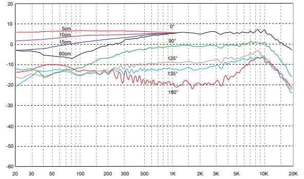
C4LC, cardioid low roll-off for close up version
