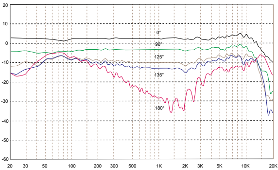
CV4F, side address, cardioid flat version
