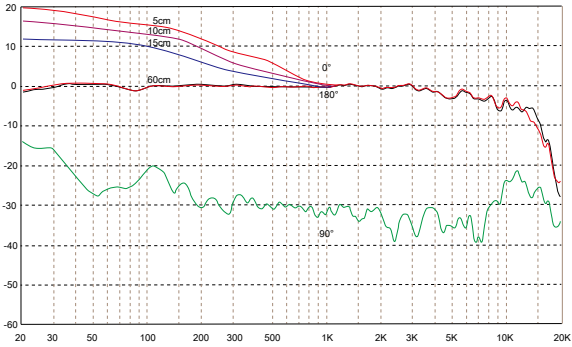
C8, figure-8 capsule
