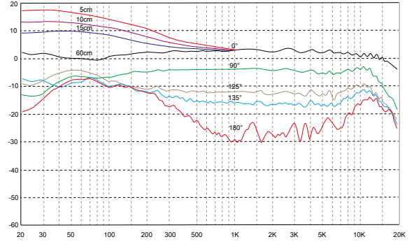
C4F, cardioid flat version
