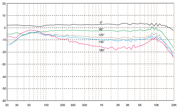
C31F, wide-cardioid flat version
