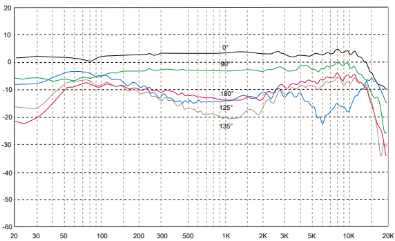
CV5F, side address, cardioid flat version
