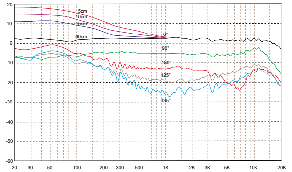
C5F, cardioid flat version
