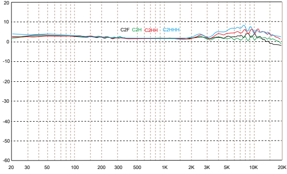
C2 series, omni capsules
