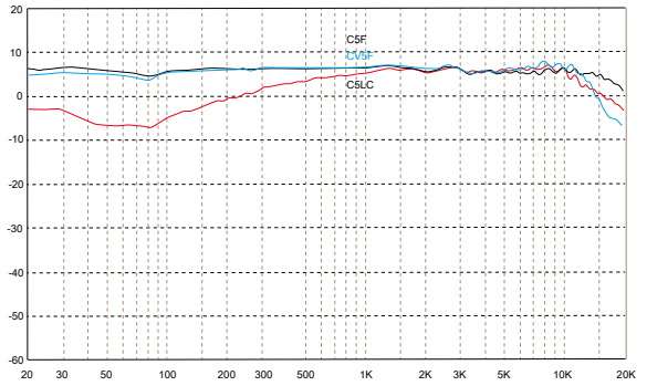
C5 series, super cardioid comparison
