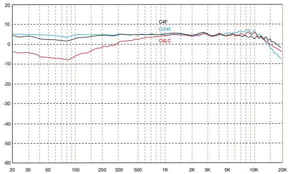
C4 series cardioid comparison
