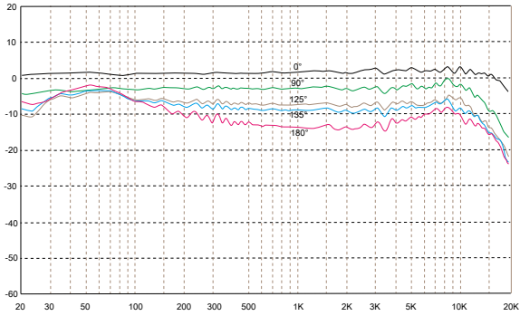
C30F, omni-cardioid flat version
