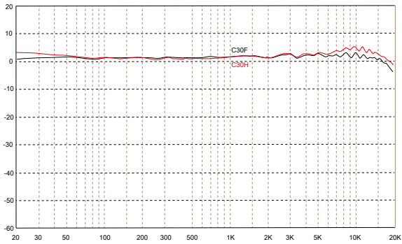
C30 series, omni-cardioid compare
