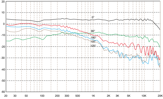
C7, interference tube, super-cardioid
