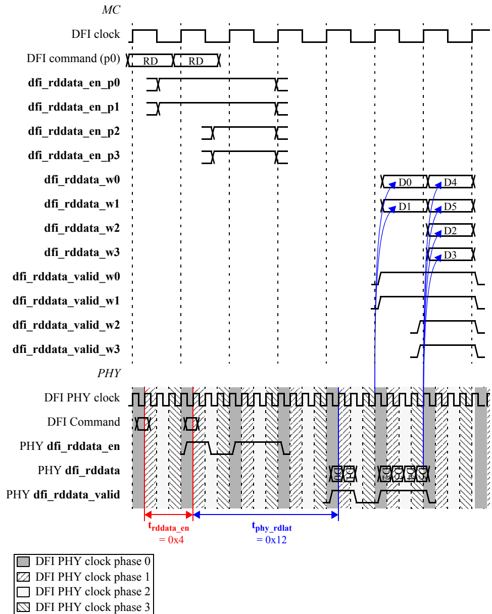
FIGURE 46. 1:4 Frequency Ratio Multiple Read Data Example
