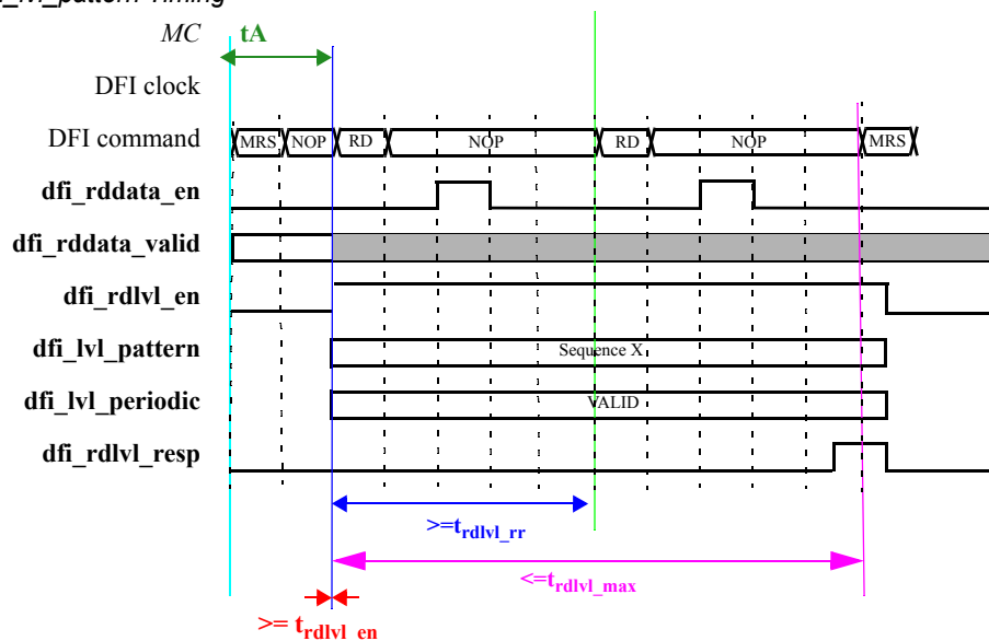
dfi_lvl_pattern Timing
