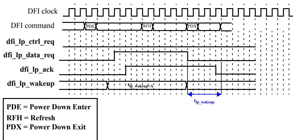
Low Power State Requiring Ongoing Use of the Control Interface
