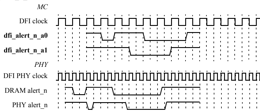
dfi_alert_n_aN with 1:2 Frequency Ratio
