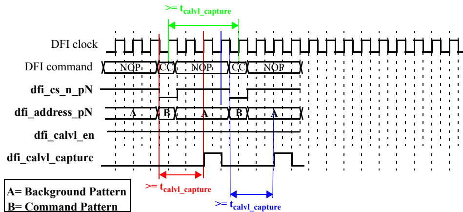
CA Training Signaling
