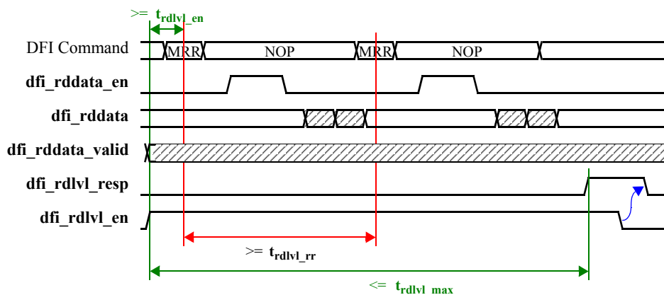
Read Training in DFI Training Mode for LPDDR3 and LPDDR2 Memory Systems
