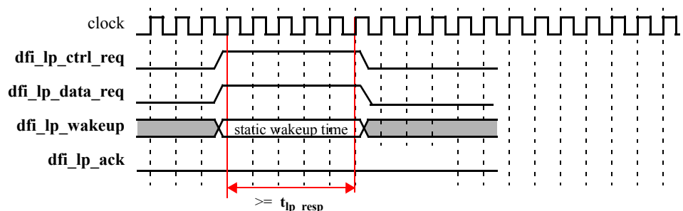
Low Power Control Request with No Response
