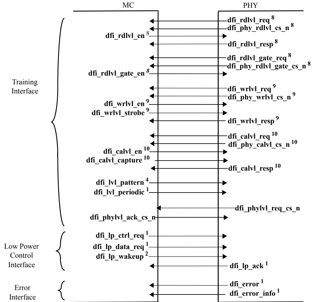
Block Diagram of Interface Signals: Training, Low Power Control and Error
