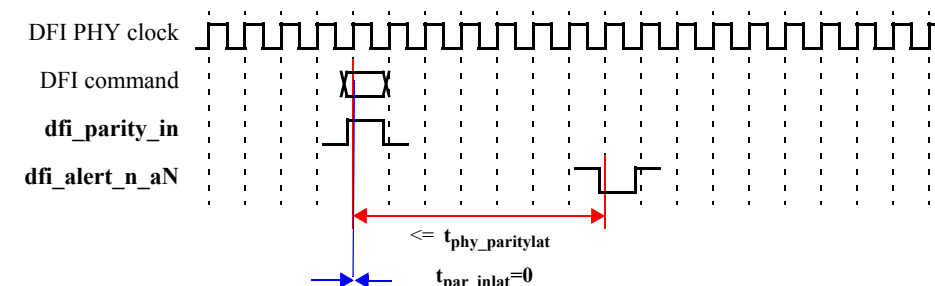
Odd Command Parity Error Example Timing Diagram
