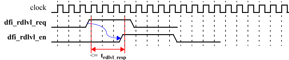
Read Data Eye Training Request Timing
