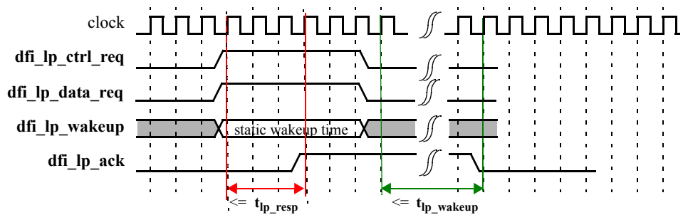
Low Power Control Handshaking Timing Diagram
