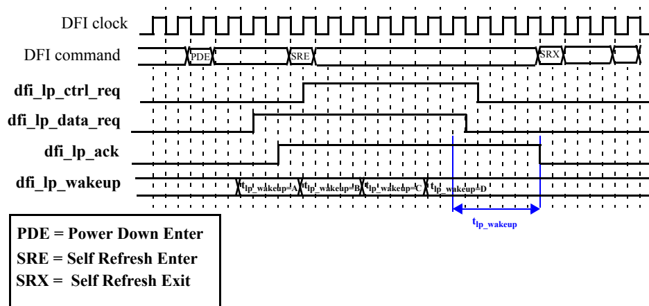
Low Power State Progressing From Requiring an active Control Interface to Functioning Independently
