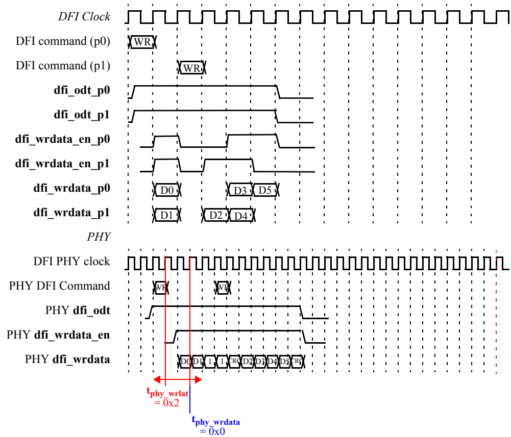
DFI Write Data Bus for PHY CRC Support Mode with Burst Chop
