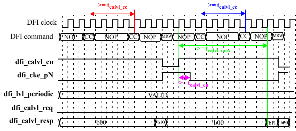
MC-Initiated CA Training Sequence
