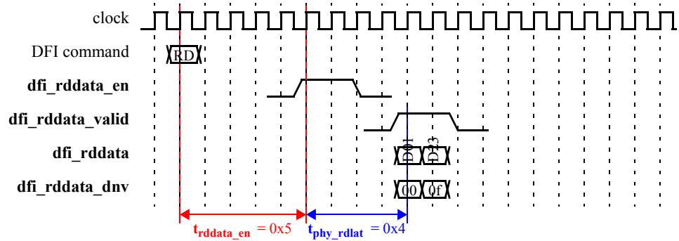
Example MRR Transactions with LPDDR3 or LPDDR2
