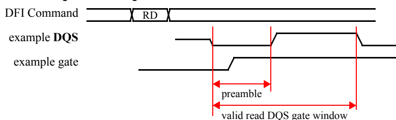
Gate Leading DQS Timing
