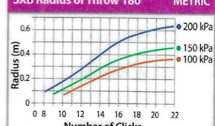
SXB Radius of Throw 180° METRIC
