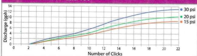
SXB Flow Rate 360° and 180°
