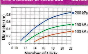
SXB Diameter of Throw 360° METRIC
