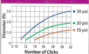
SXB Diameter of Throw 360°
