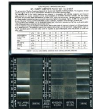
Surface Roughness Compariter
