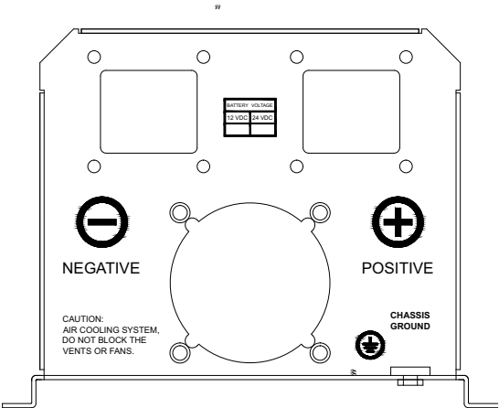
600 TO 500 W MODELS SIDE VIEW
