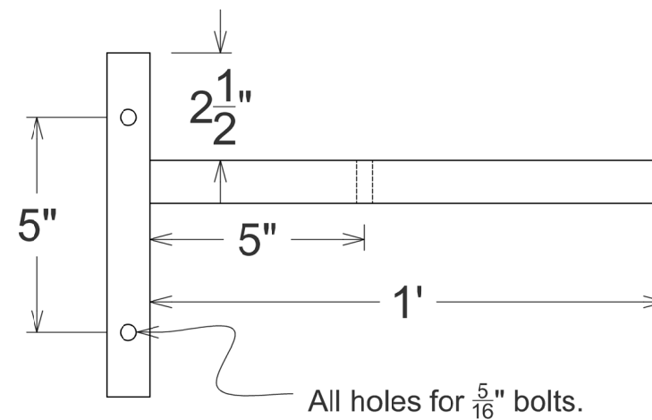
SUPPORT BRACKET MAKE 4 (SCALE: 3" = 1')
