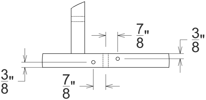
DETAIL B SCALE 3" = 1'-0"
