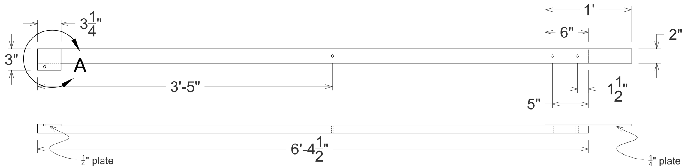
SUPPORT SPAR MAKE 4 (SCALE: 1-1/2" = 1')
