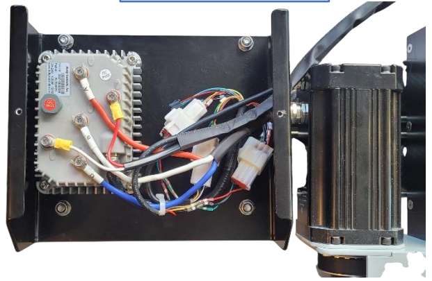
DRIVER CONTROLLER
