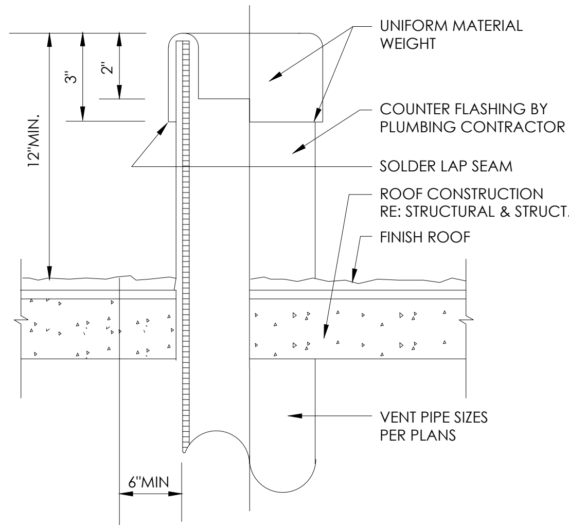
VENT THRU ROOF DETAIL
