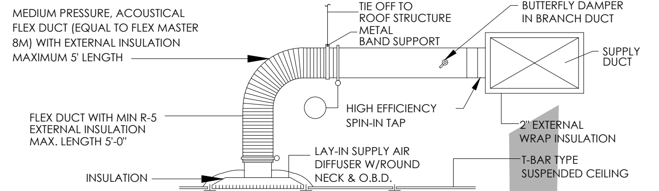
SUPPLY AIR DIFFUSER CONNECTION
