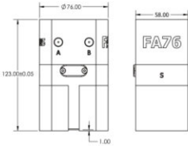
FA76 Standard Flat Pole
