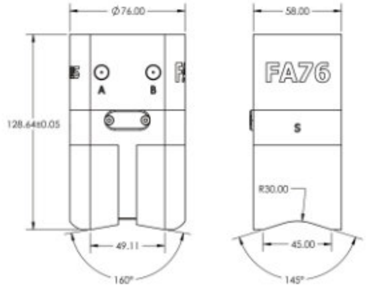
FA76 Standard V Pole
