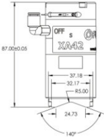
XA42 Standard V Pole Kit Dimensions (P/N: 4060051)
