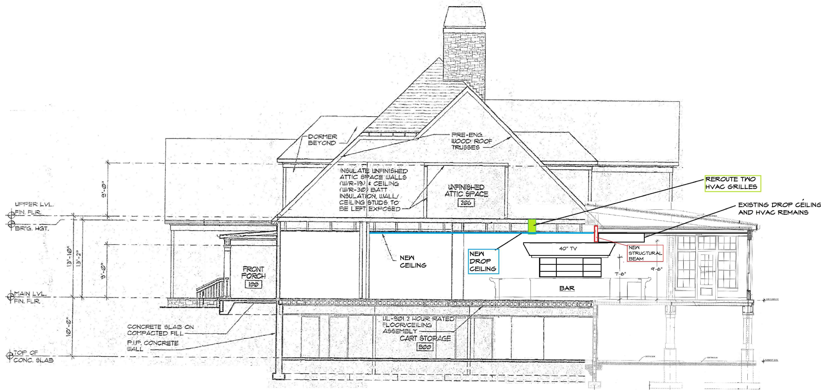
SECTION WITH EXISTING DROP CEILING
