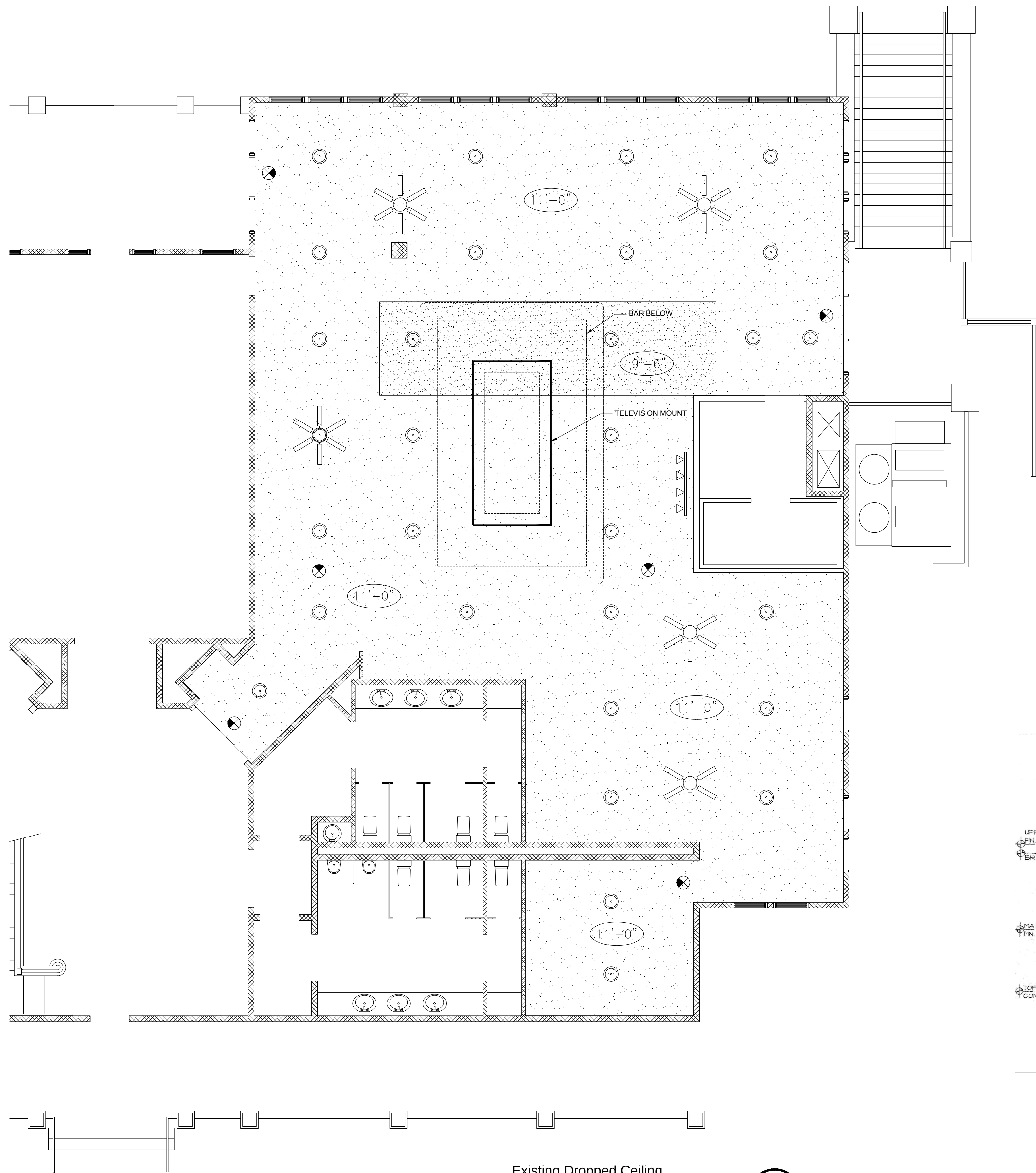
Existing Dropped Ceiling Reflected Ceiling Plan SCALE: 3/16" = 1'-0"
