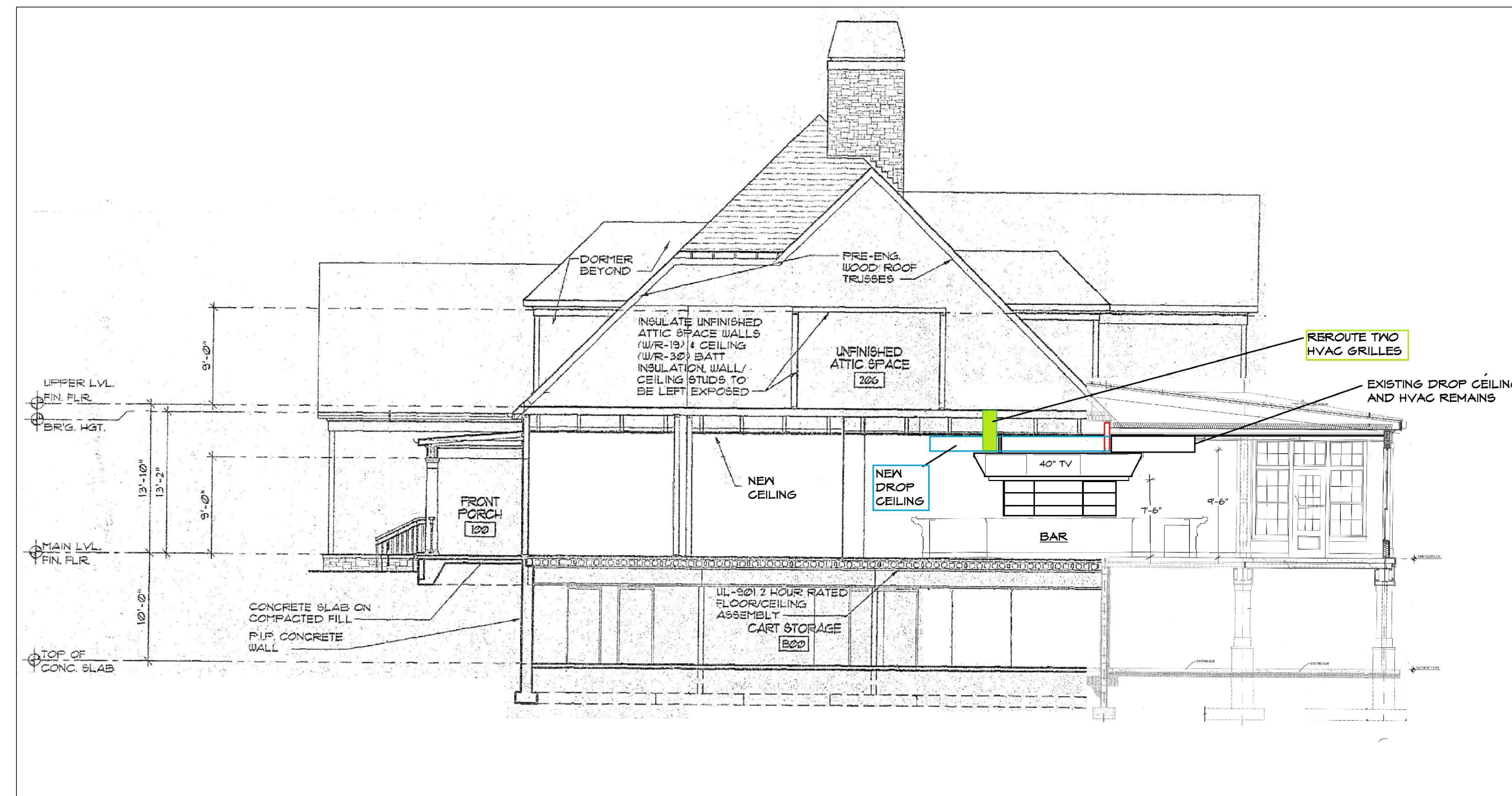
SECTION WITH LARGE DROP CEILING
