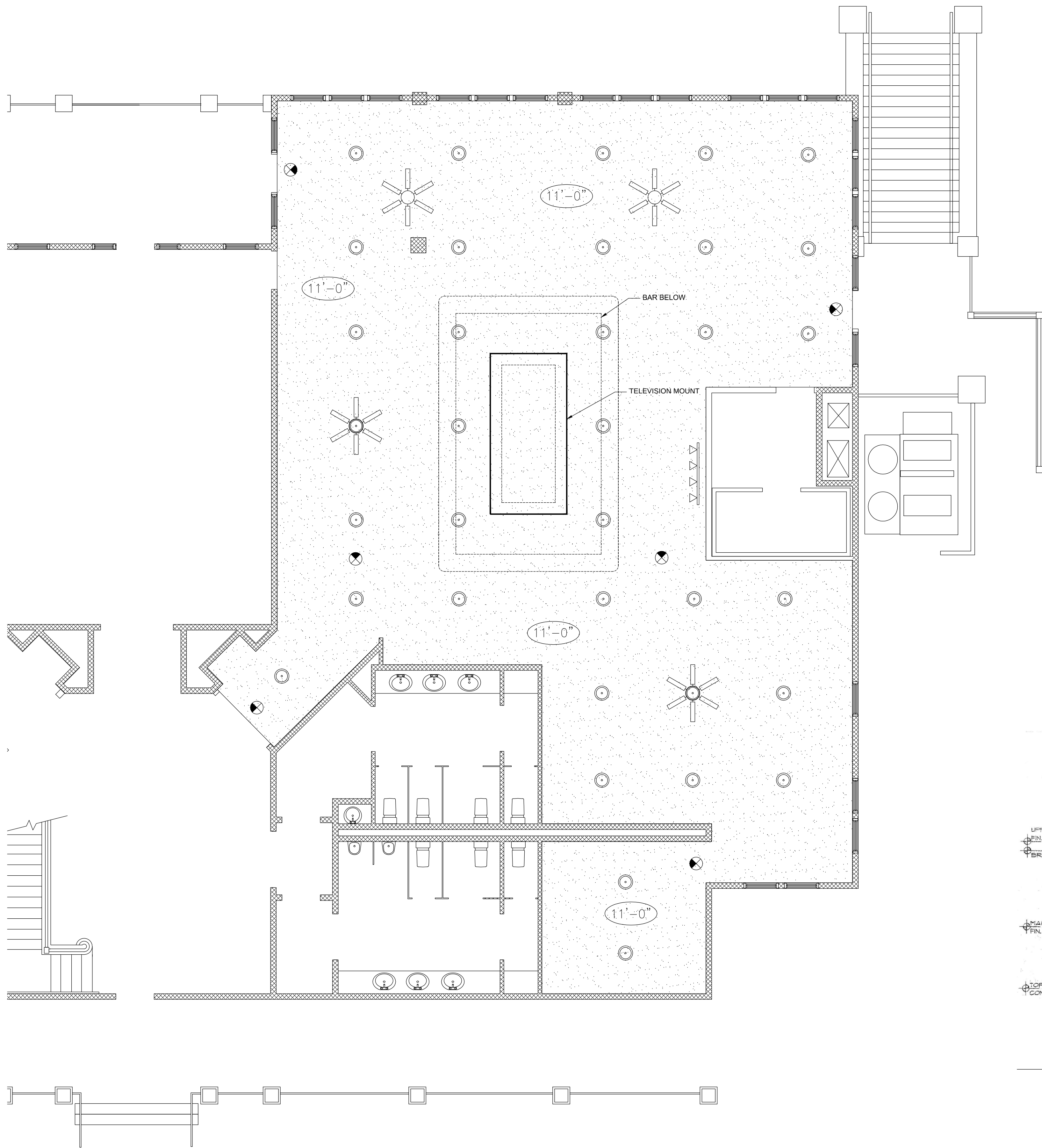
Flat Ceiling Reflected Ceiling Plan SCALE: 3/16" = 1'-0"
