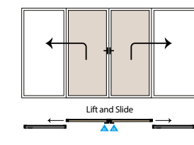
4 Pane - 2 Slide
