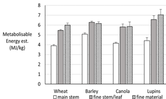
Figure 4. The estimated metabolisable energy content (MJ/kg DM) of chaff collected from winter crop stubbles in Western Australia (2018)
