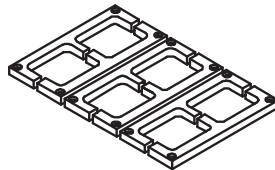
Stripper Shoes
