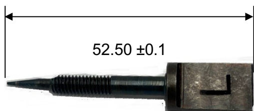
REF.39 - P. N° 43-1046 NEEDLE LOW SPEED
