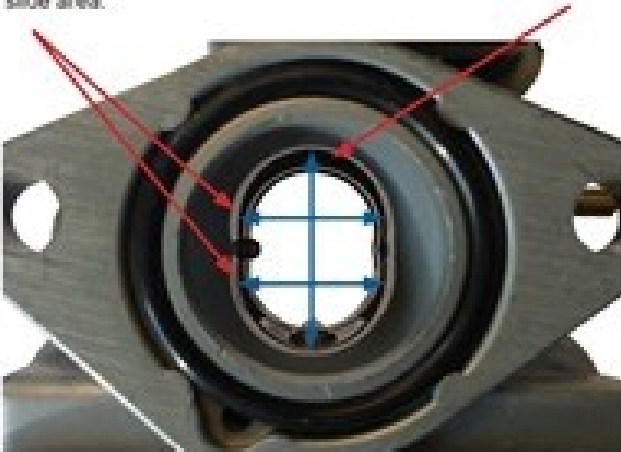
Venturi Horizontal Measurement (widest part) - .615" no-go can't pass into slide area.
