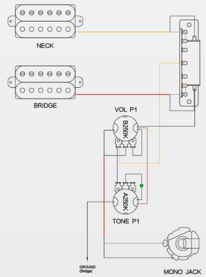
H-H,1V/1T,3-Way Selector
