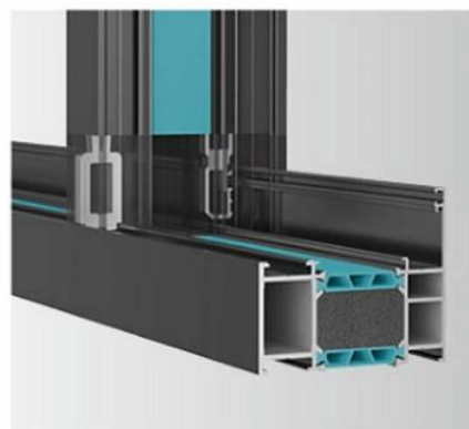
Pin And Mullion Connection
