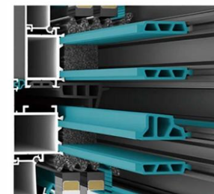
PA66 Nylon Insulation Strip
