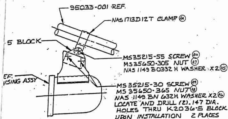
(A2) VIEW B-B KATE COMPASS ON 95033-001 SUPPORT TUBE PER OWNERS REQUEST
